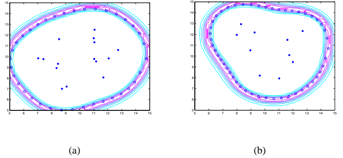
Fig. 4. Two examples of entrapping stationary targets with multiple robots using the H-GRN, where the targets are denoted by a dot and the robots by a circle. The contours denote the concentration distribution of protein g_3 . (a) 36 robots entrap 15 targets, (b) 49 robots entrap 10 targets.
