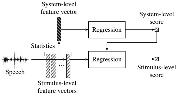
Figure 2: Hierarchical prediction system: the predicted system-level score is used as a feature for stimulus-level prediction.
