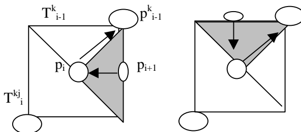
FIGURE 9. Fictitious vertex dependencies
