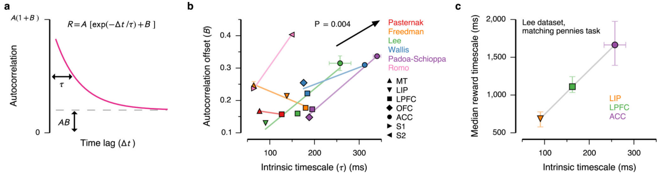
Figure 2. Links between intrinsic timescale and longer functional timescales. (a) Autocorrelation offset ( B ) reflects the strength of contributions with long timescales, which do not decay substantially within the fixation epoch. (b) Autocorrelation offset increases with intrinsic timescale. Colored lines show trends for individual datasets. The arrow shows the slope of dependence from a regression analysis (slope m = 0.8 \pm 0.2 kHz). (c) In the Lee dataset, we previously measured timescales characterizing the decay of modulation of single-neuron firing rates by reward events, while monkeys performed a competitive decision-making task 11 . The ordering of areas by reward timescale aligns with the ordering by intrinsic timescale. Error bars mark s.e.
