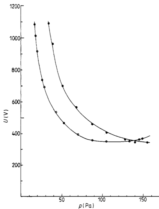
Figure 2. Operating voltage as a function of buffer gas pressure for an aluminium-argon hollow cathode. Parameter is the discharge current I (A): ○, 1; ●, 2.
