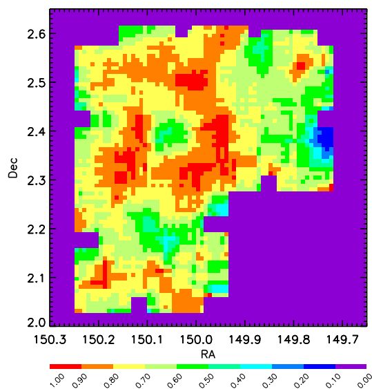
Fig. 11. RaDec Sampling rate before normalization, showing the spatial variation of the TSR due to the sky inhomogeneities in our survey coverage. Comparing this figure with Fig. 5 it is possible to see that the highest density region where the richest structure is located suffers from a slight relative under-sampling, despite having been targeted by four different pointings.
