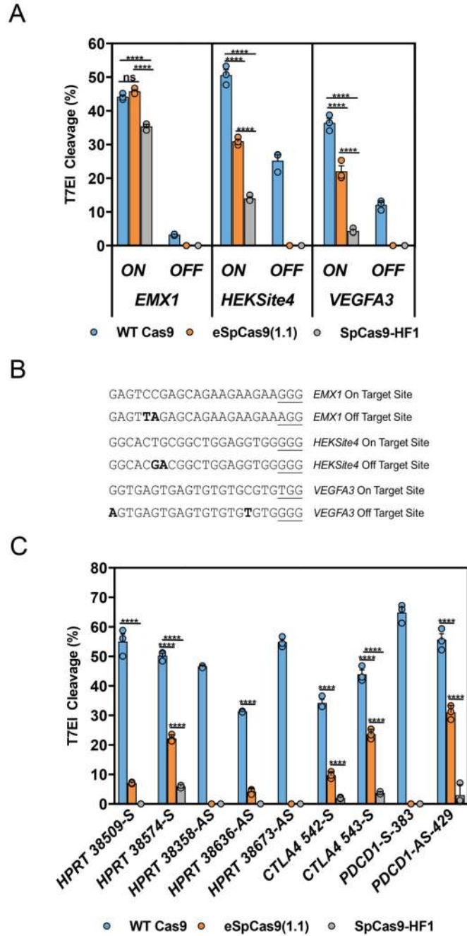
Figure 1. On-target activity of high-fidelity Cas9 mutants in human cells with ribonucleoprotein (RNP) delivery.
