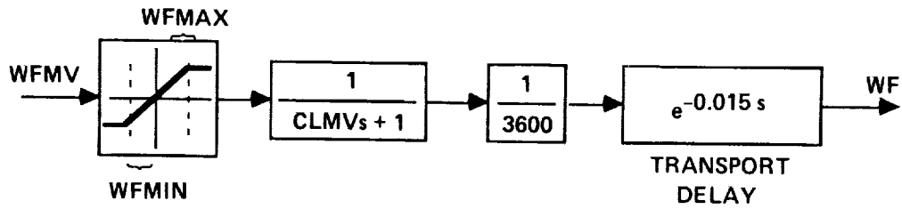
Figure C19.- Fuel flow metering valve.
