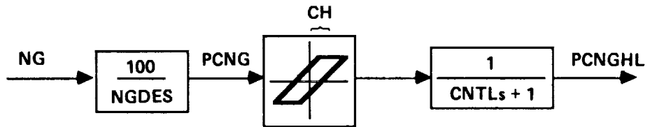
Figure C15.- NG spool sensor dynamics.
