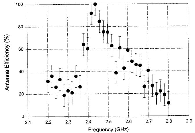
Fig. 7. Radiation efficiency versus frequency.
