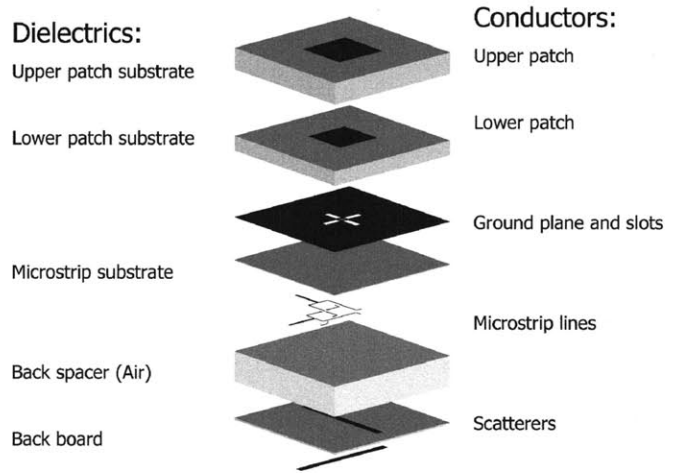
Fig. 1. Antenna architecture.
