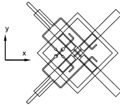
Fig. 2. Conductors views with coordinate system indication.
