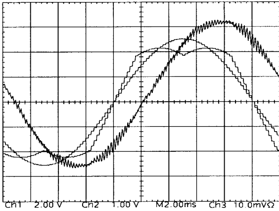
Fig. 15. Experimental SVPWM modulation wave, its fundamental component, and the motor current waveforms ( M_i = 0.79 , 49 Hz, 50% T_{eR} ). Scaling: 2 A/div, 2 V/div, and 2 ms/div.
