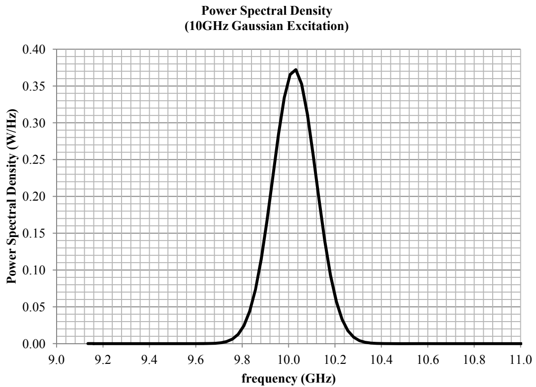
Figure 18. Power spectral density of 10GHz Gaussian excitation
