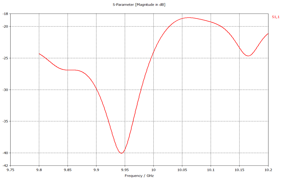
Figure 35. S11 Measurement for Lens 1 at y = 500 mm.
