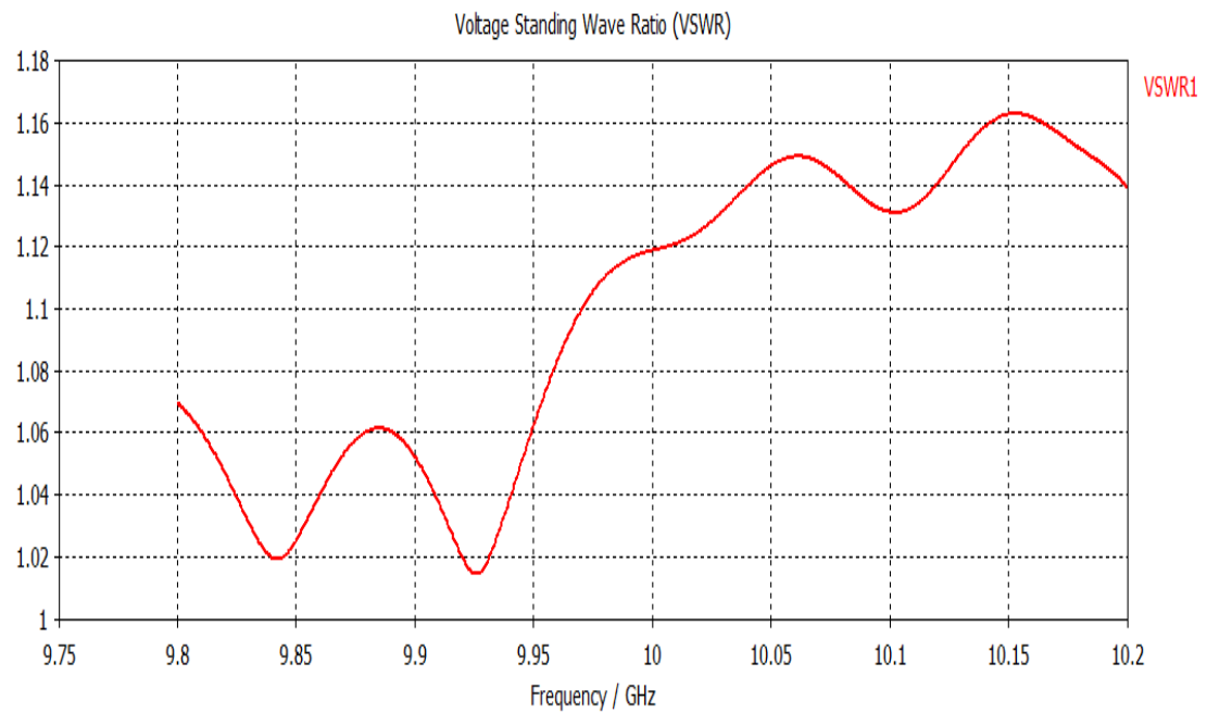
Figure 38. VSWR with lens 1 at y = 700mm
