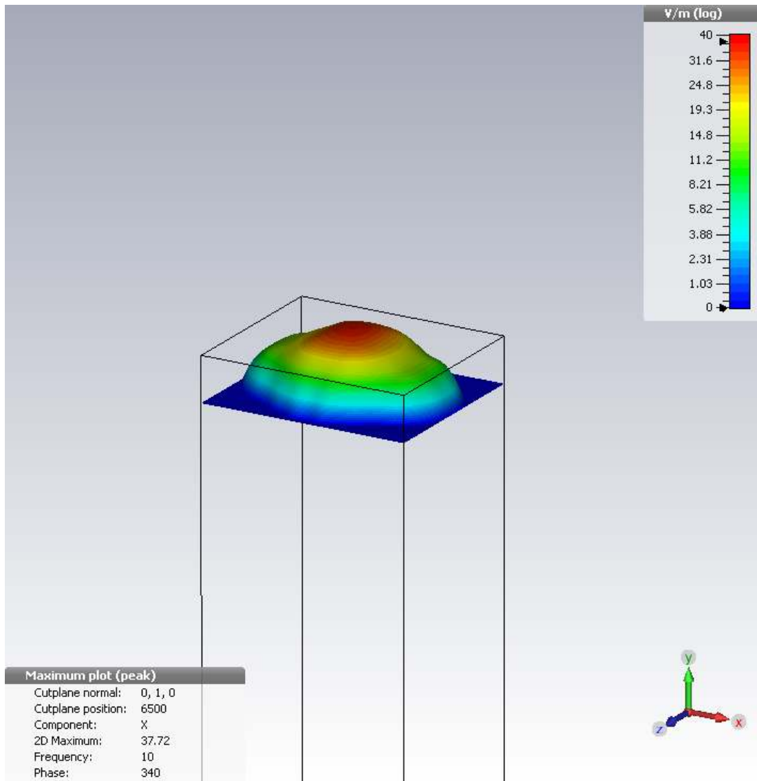
Figure 41. “Carpet” Representation of Electric Field (Ex) at y = 6500mm (Narrow Beam)
