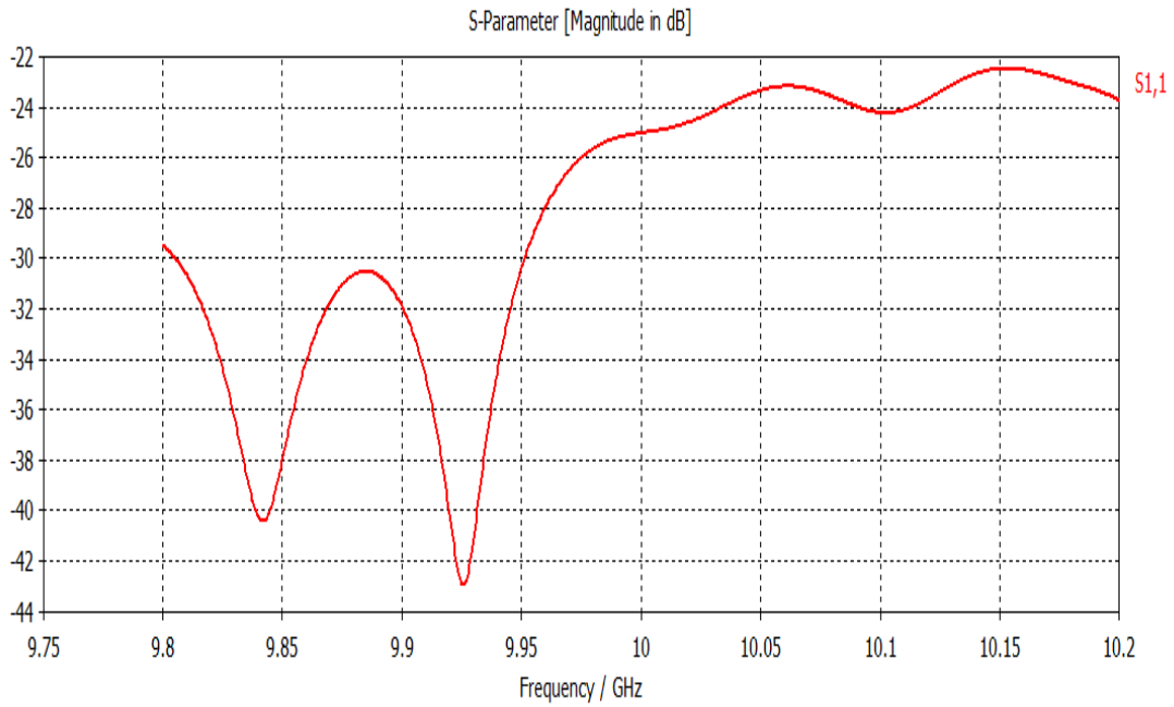
Figure 37. S 11 of Horn/Lens combination with lens at y = 700mm [vertical axis: S 21 (dB)]
