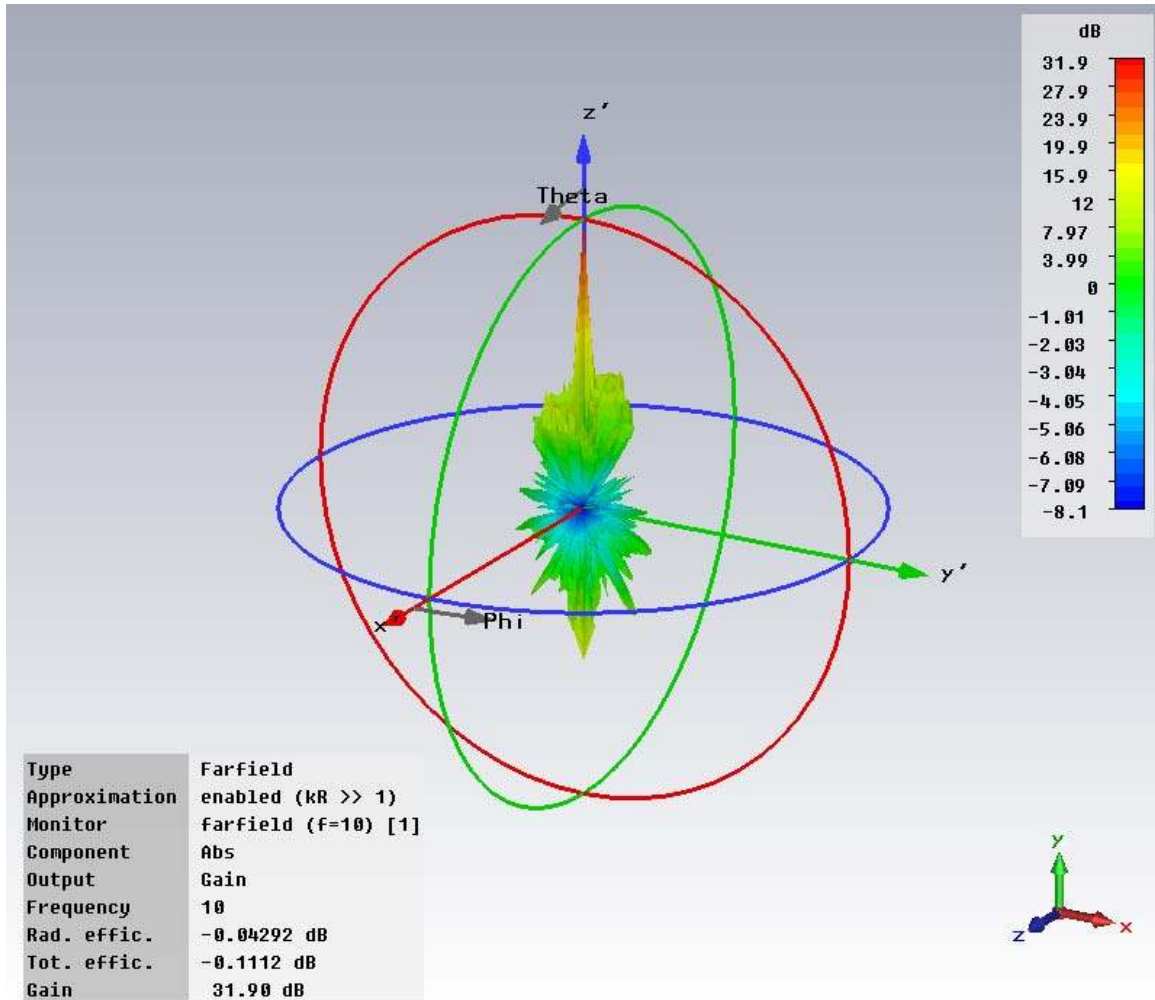
Figure 56. 3-D Radiation Pattern (Broad Beam)
