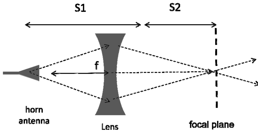
Figure 6. Focus of beam to an Airy Disc in the focal plane when S_1 > f
