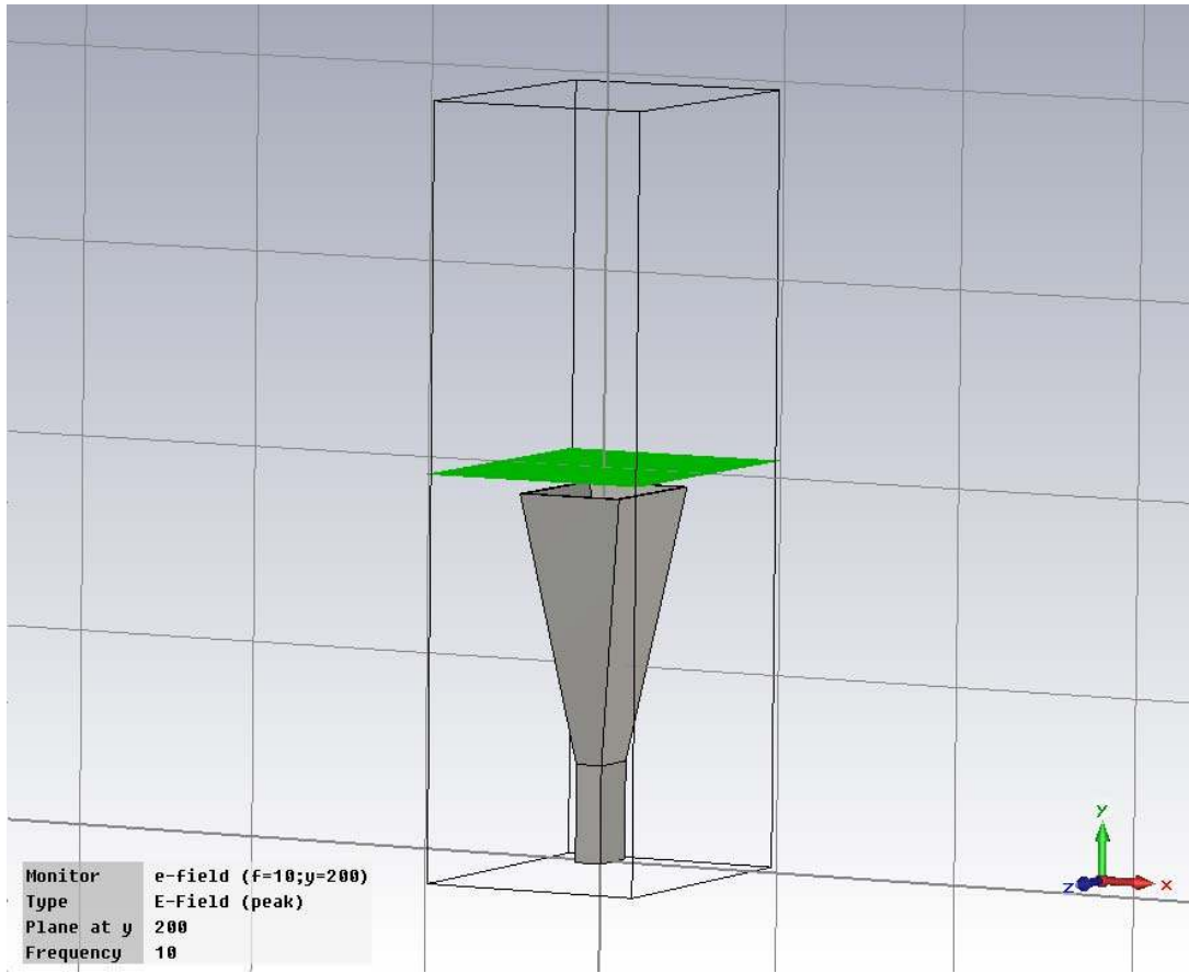
Figure 92. X-Band Horn with Field Monitor in the Near Field ( y = 200\text{mm} )
