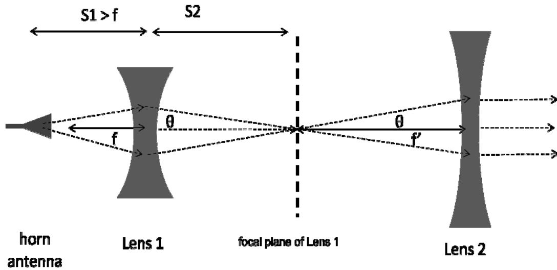
Figure 7. Collimation of beam by placing a second lens, with focal length f' , one focal length away from the focal plane of Lens 1
