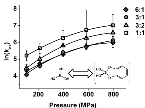
Figure 3. \ln(k_{\text{ex}}) as a function of pressure for various H 3 BO 3 (0.3 M)/catechol solution compositions at T = 323 K. The data are fitted to the quadratic Equation (3) with the resulting apparent activation parameters compiled in Table 1. The inset shows the two 11 B species used to calculate k ex from the 11 B NMR spectra acquired on the high-pressure cell NMR probe. The error bars indicate the standard error of each datum.
