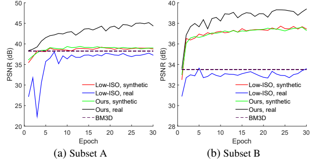
Figure 8: Testing results of DnCNN [33] using two types of ground truth (post-processed low-ISO and our ground truth images) and two types of noise (synthetic and real) on two random subsets of our dataset (see Table 2). Training with our ground truth on real noise yields the highest PSNRs.
