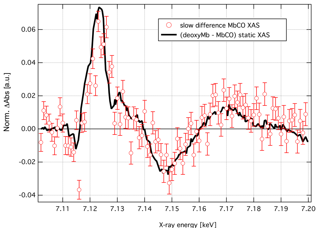
FIG. 12. (Color online) Transient XAS of 2 mM MbCO collected in fluorescence yield mode. The sample was excited at 125 \text{ mJ/cm}^2 laser fluence. The black curve represents the difference XAS based on the static spectra of deoxyMb and MbCO assuming an excitation yield of 21%.
