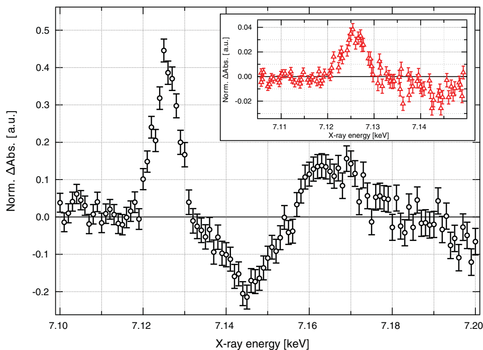
FIG. 8. (Color online) Average of 10 transient XAS scans 50 ps after excitation, of a 1 mM [\text{Fe}(\text{bpy})_3]^{2+} solution excited with a pump fluence of 150 \text{ mJ}/\text{cm}^2 . The inset shows a single transient XAS scan of a 25 mM aqueous solution of [\text{Fe}(\text{bpy})_3]^{2+} at 50 ps delay and collected in fluorescence yield mode with a pump fluence of 13 \text{ mJ}/\text{cm}^2 .
