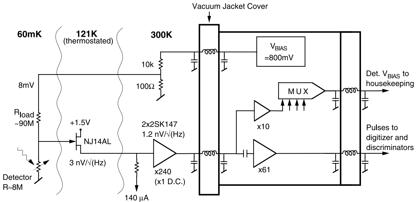
FIG. 5.—Analog electronics chain for a single pixel. These circuits are inside the cryostat or mounted on the top cover.
