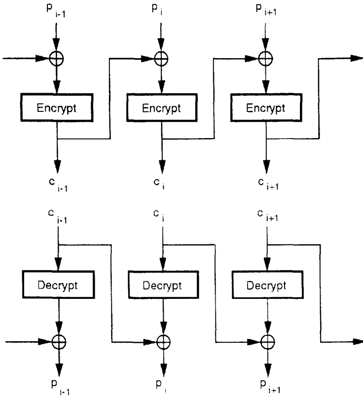
Fig. 4. Cipher Block Chaining
