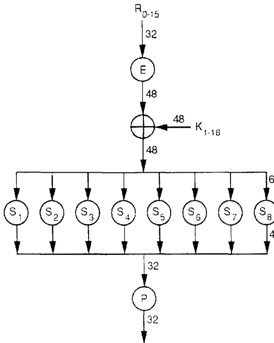
Fig. 3. Expanded Version of Function f
