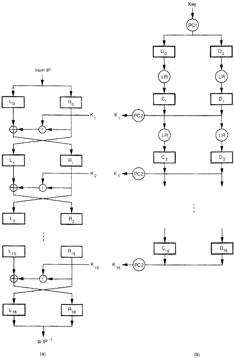
Fig. 2. Expanded Version of the 16 Iterations (a) and the Key Schedule (b) for Encryption
