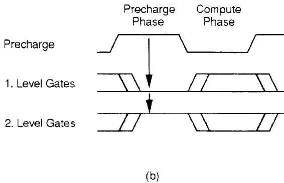
Fig. 7. Precharged NOR-NOR Logic (a) and Timing (b)
