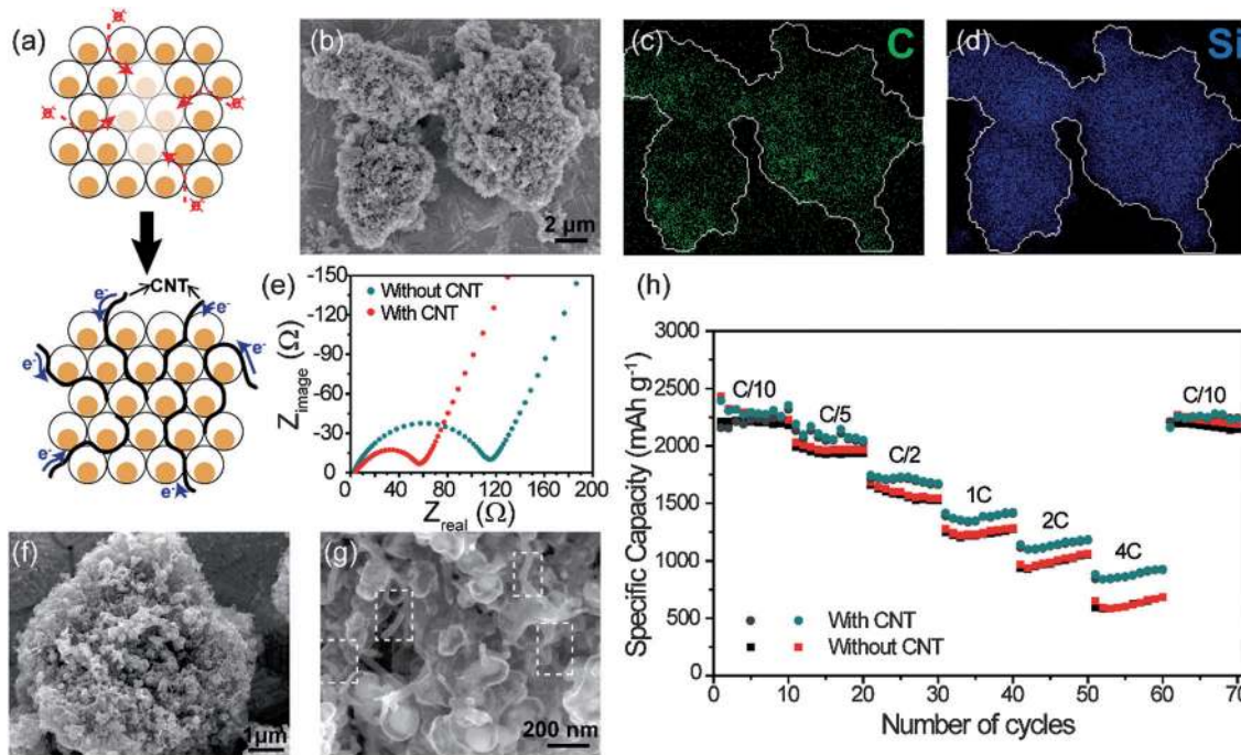
Fig. 4 CNT-embedded nano-Si SC for improved intracluster conductivity. (a) Schematically shows electron transport in SC with and without CNTs. CNTs assist radial electron transport and activate more active materials. (b) SEM image of SC before carbon coating. Corresponding energy-dispersive X-ray spectroscopy maps of (c) carbon distribution and (d) silicon distribution. (e) Nyquist plots of nano-Si SC with/without embedded CNTs after the completion of first delithiation. (f) Typical SEM image of CNT-embedded nano-Si SC. (g) Magnified SEM image showing surface distribution of CNTs and Si nanostructures. (h) Rate capability of SC with/without embedded CNTs with various rates from C/10 to 4C.
