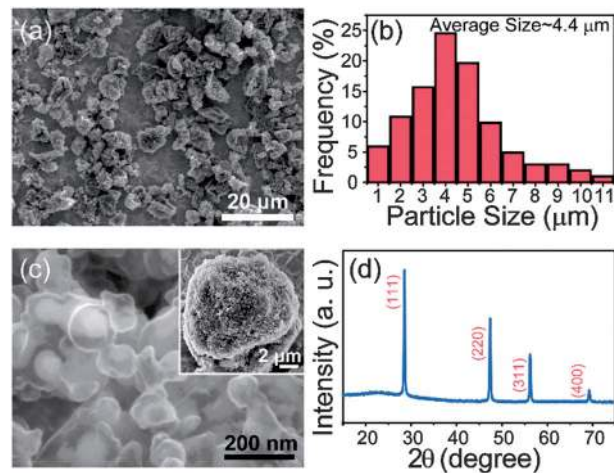
Fig. 2 Characterization of nano-Si SC. (a) Low-magnification SEM image showing the size distribution of SC. (b) Statistical analysis of the distribution of SCs' size based on (a). (c) Magnified SEM image of the surface of SC showing the well-defined void space as well as intact carbon framework. Inset image shows one typical cluster. (d) X-ray diffraction pattern of as-obtained nano-Si SC powders.
