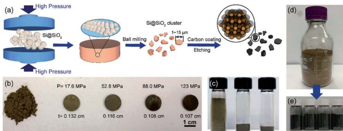
Fig. 1 Mechanical fabrication of the nanostructured silicon (nano-Si) secondary cluster. (a) Schematic illustration of the mechanical-based nano-Si SC fabrication process. (b) Produced pellets under various pressures and their evolution of thickness under increasing applied pressure. Left shows the pristine powder before pressing. Each contains 0.25 g of \text{Si@SiO}_2 . (c) Volume comparison on 0.4 g samples in 4 mL vials. From left to right, Si nanoparticle, micro-emulsion produced cluster, and mechanically produced cluster, respectively. (d) Starting materials of \text{Si@SiO}_2 powders. (e) 20.12 g of final product (bottom) produced at lab scale from starting powders shown in (d).
