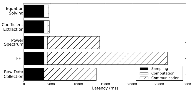
Fig. 16. The latency of sensor data collection and processing
