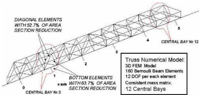
Fig. 12. Truss finite element model
