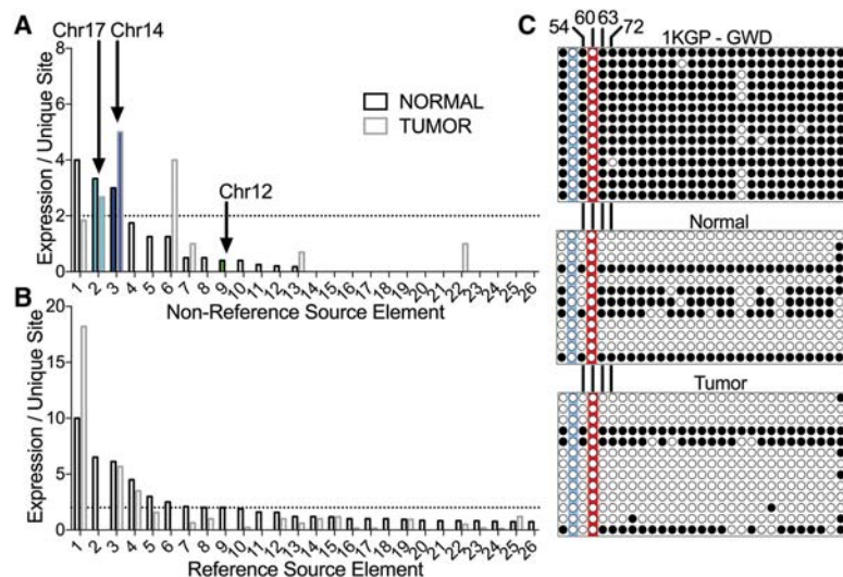
Figure 4. FL-L1Hs source element expression in normal and tumor tissues. The unique interior mutation profiles of FL-L1Hs elements in the patient's genome (Fig. 2) were used to quantify expression of the 31 nonreference FL-L1Hs source elements including the Chr 17, Chr 14, and Chr 12 source elements (A) and the remaining 264 reference FL-L1Hs source elements in the patient's genome, using strand-specific RNA-seq (B) (Supplemental Table S3; Methods). Expression for each element is depicted in the normal and tumor tissues as the mean number of independent reads covering all mutations unique to a FL-L1Hs source element. Expression of FL-L1Hs source elements that could not be differentiated from the expression of the surrounding gene in the same orientation were excluded from this analysis (A, n = 4 ; B, n = 37 ) (Supplemental Table S3). The horizontal dotted lines represent a cutoff where the mean = two traces per unique site, and a total of 10 elements were expressed above this level. (C) DNA methylation analysis of the Chr 17 source element promoter. The top panel displays bisulfite sequencing results for the control 1000 Genomes Project (1KGP) sample (GWD sample HG02583, which is heterozygous for the Chr 17 element; Coriell). The two panels below show the results of bisulfite sequencing in the normal and tumor tissues of the CRC patient. Each circle represents a CpG site in the promoter (for a total of 29 CpGs at positions: 21, 37, 54, 60, 63, 72, 102, 137, 155, 160, 164, 166, 171, 181, 205, 231, 251, 255, 269, 284, 293, 305, 317, 320, 327, 351, 363, 369, 377 relative to the reference L1.3 sequence; GenBank ID L19088). White circles indicate no DNA methylation; black circles indicate DNA methylation. The red highlighting indicates the CpG at position 60 that previously was shown to be critical for repression of the L1 promoter by DNA methylation (Hata and Sakaki 1997). This CpG is mutated in the Chr 17 element (G61A). The three remaining CpG sites that are critical for repression of the L1 promoter by DNA methylation also are indicated (positions 54, 63, 72) (Hata and Sakaki 1997). The blue highlighting indicates a CpG to TpG mutation at position 37 that destroys an additional CpG in the promoter region.
