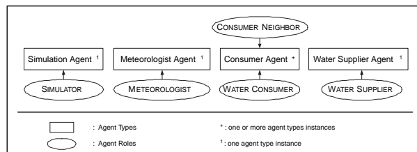
Figure 5. DAWN agent model
