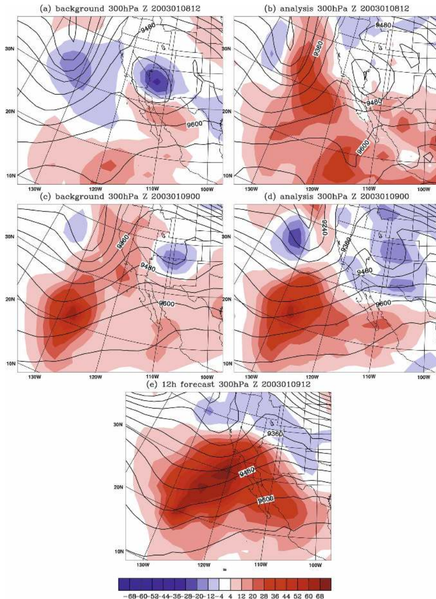
FIG. 9. The difference of the analysis and the first guess for the 300-hPa geopotential height between the 3DVAR and the hybrid from 1200 UTC 8 Jan to 1200 UTC 9 Jan 2003 every 12 h. Difference of the (a) background and (b) analysis at 1200 UTC 8 Jan 2003, the (c) background and (d) analysis at 0000 UTC 9 Jan 2003, and the (e) difference of the 12-h forecast at 1200 UTC 9 Jan 2003. Black contours are the 300-hPa geopotential height (m) for the hybrid. Color shades are the difference (3DVAR minus hybrid) of the 300-hPa geopotential height (m).
