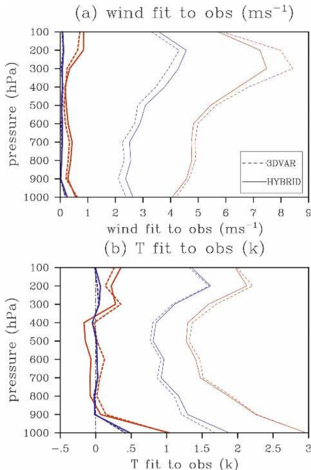
FIG. 2. Vertical profiles of the rms fits of the 12-h forecasts (red thin line) and analysis (blue thin line) to the radiosonde observations and biases of the 12-h forecasts (thick red line) and analysis (thick blue line) fits to the radiosonde observations for 3DVAR (dotted) and hybrid with 1/\beta_1 = 0.5 and S_e = 2828\text{km} : (a) wind and (b) T .
