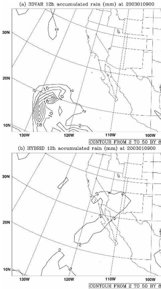
FIG. 10. The 12-h forecasts of the accumulated precipitation valid at 0000 UTC 9 Jan 2003 for (a) 3DVAR and (b) hybrid.
