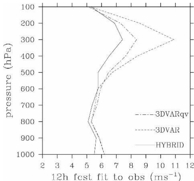
FIG. 6. Vertical profiles of the rms fit of the 12-h wind forecast valid at 1200 UTC 9 Jan 2003 to the radiosonde observations over the verification domain for hybrid with 1/\beta_1 = 0.5 and S_e = 2828 km (solid line), 3DVAR (dotted line), and 3DVAR whose water vapor mixing ratio analysis was replaced by that of the hybrid at 1200 UTC 8 Jan 2003 (dash-dotted line).
