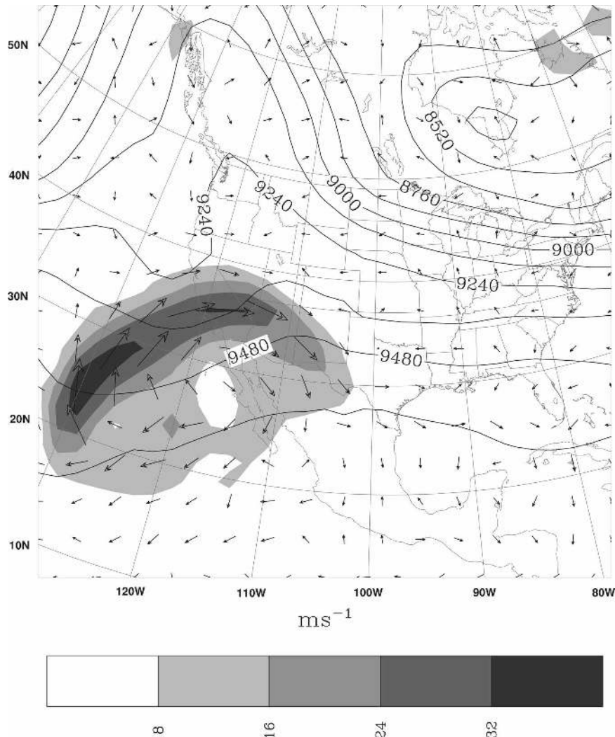
FIG. 7. The difference of the 12-h wind forecast between the 3DVAR and the hybrid with 1/\beta_1 = 0.5 and S_e = 2828 km valid at 1200 UTC 9 Jan 2003. Solid lines are the 12-h 300-hPa height forecast of the hybrid (m). Vectors are the wind forecast difference (3DVAR – hybrid). The shades are the magnitude of the wind forecast difference.
