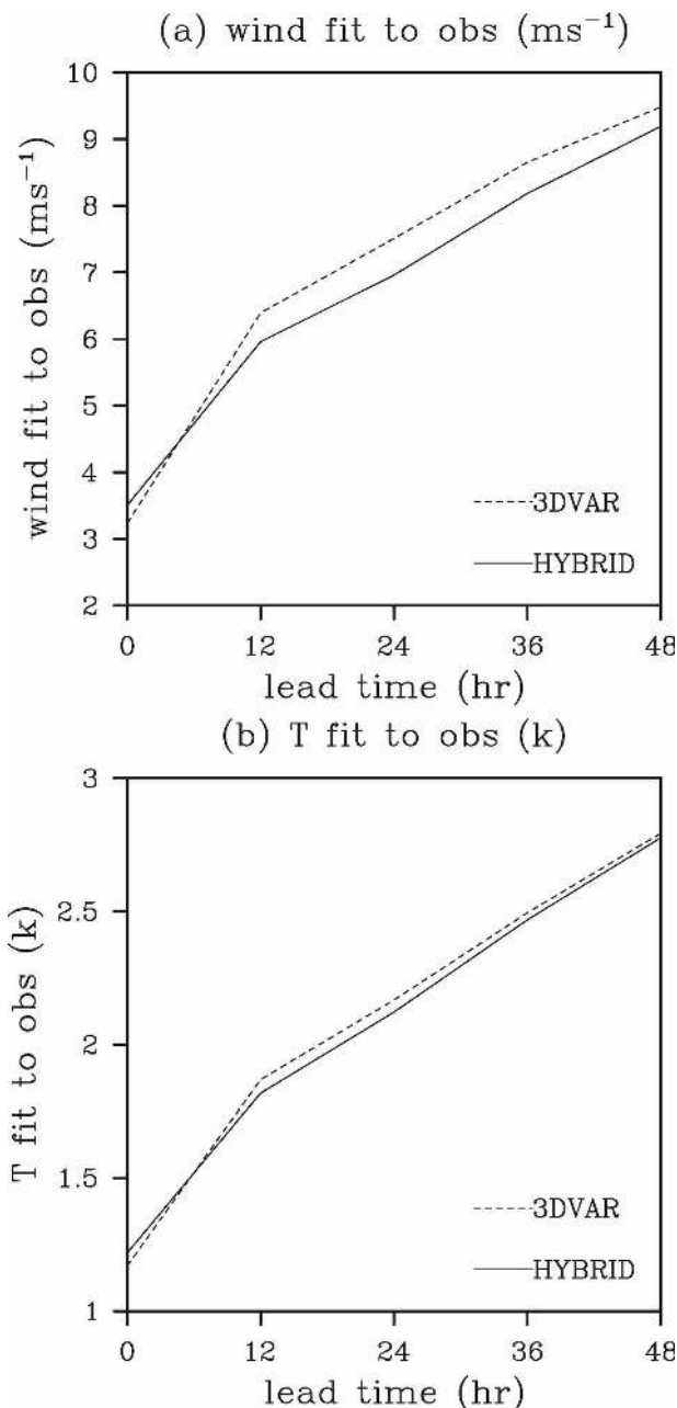
FIG. 3. The rms fit of the forecast to observations as a function of forecast lead times up to 48 h for the hybrid (solid line) and the 3DVAR (dotted line) for (a) wind and (b) T .
