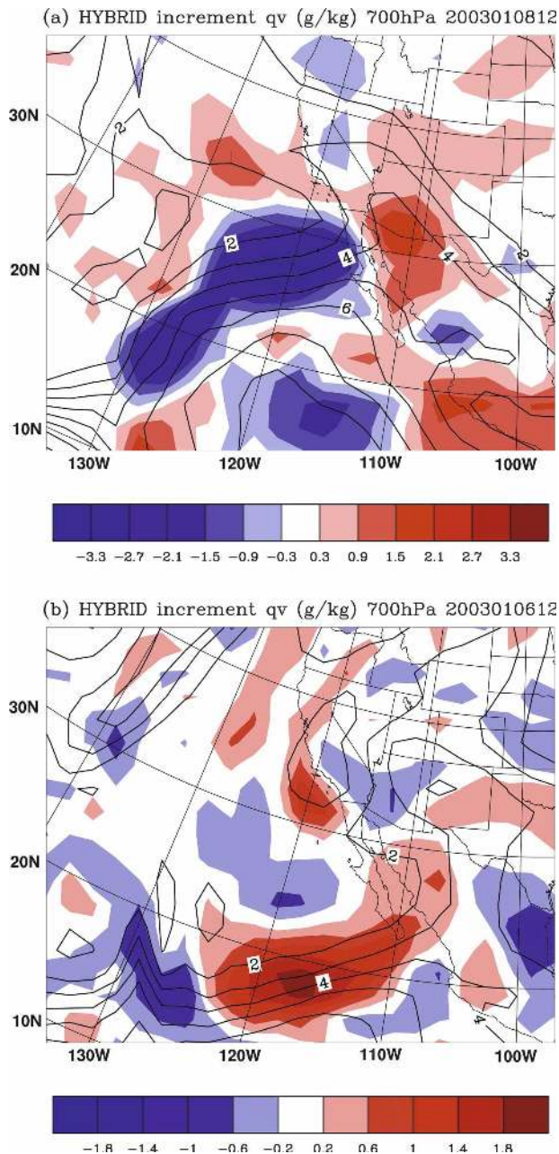
FIG. 12. The 700-hPa water vapor mixing ratio increment by the hybrid at (a) 1200 UTC 8 Jan and (b) 1200 UTC 6 Jan 2003. Black lines are the first guess of the 700-hPa water vapor mixing ratio. Color shades are the increment of the mixing ratio by assimilating radiosonde wind and T observations.
