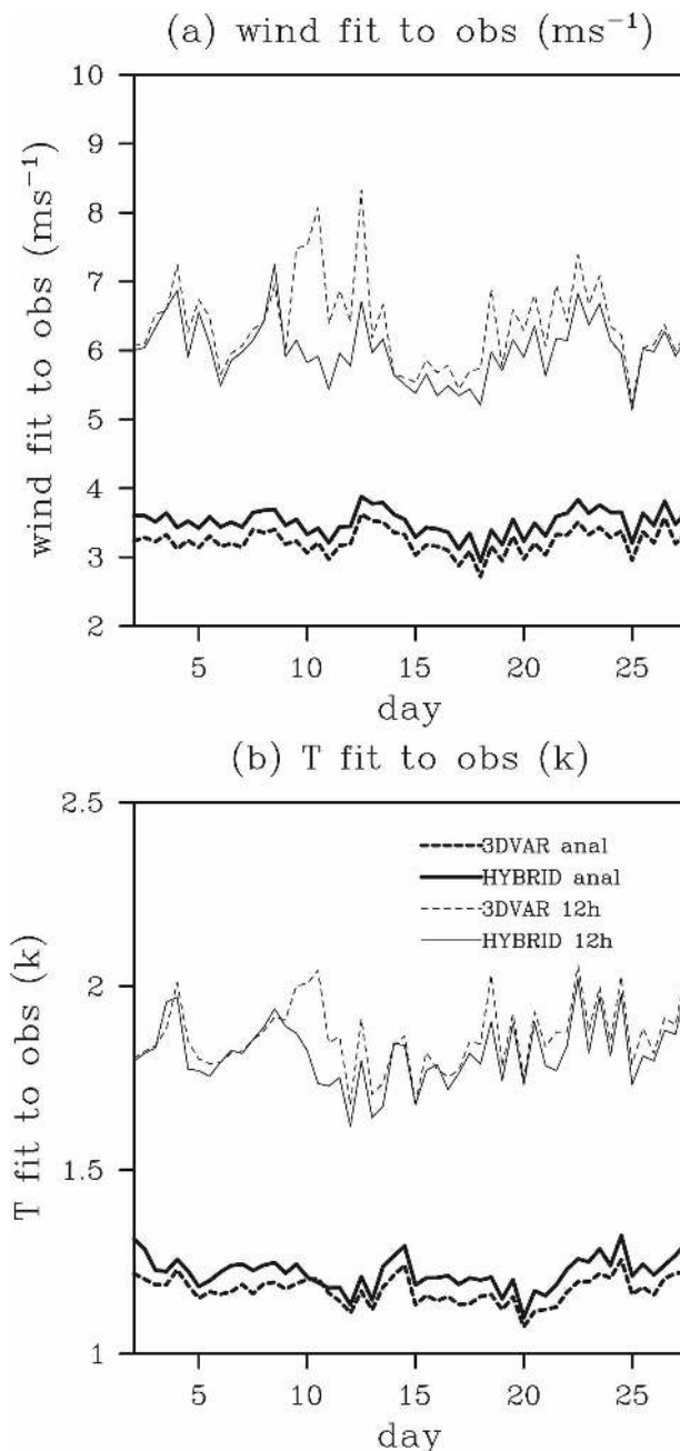
FIG. 1. Time series of the rms fit of the 12-h forecasts to the radiosonde observations (thin lines) and the rms fit of the analysis to the radiosonde observations (thick lines) over the verification domain for 3DVAR (dotted) and the hybrid with 1/\beta_1 = 0.5 and S_e = 2828 km (solid): (a) wind and (b) temperature ( T ).
