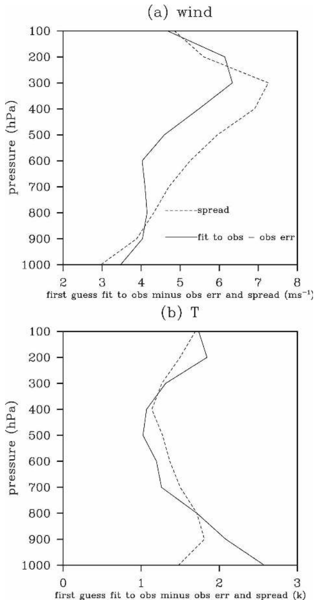
FIG. 5. Vertical profiles of the ETKF ensemble spread (dotted line) vs the square root of the innovation variance – observation error variance (solid line) for (a) wind and (b) T .
