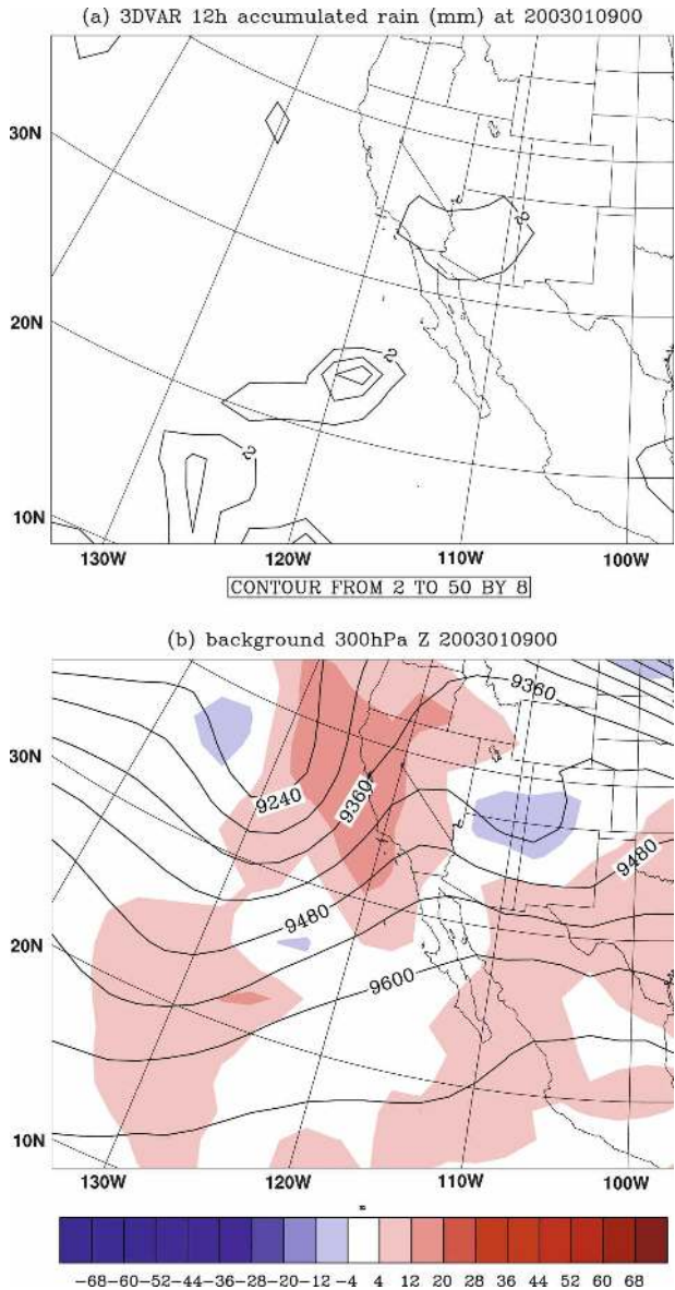
FIG. 11. (a) As in Fig. 10a, and (b) as in Fig. 9c, but the plots represent the forecast simulations in which the 3DVAR water vapor mixing ratio analysis at 0000 UTC 9 Jan 2003 was replaced with that of the hybrid.
