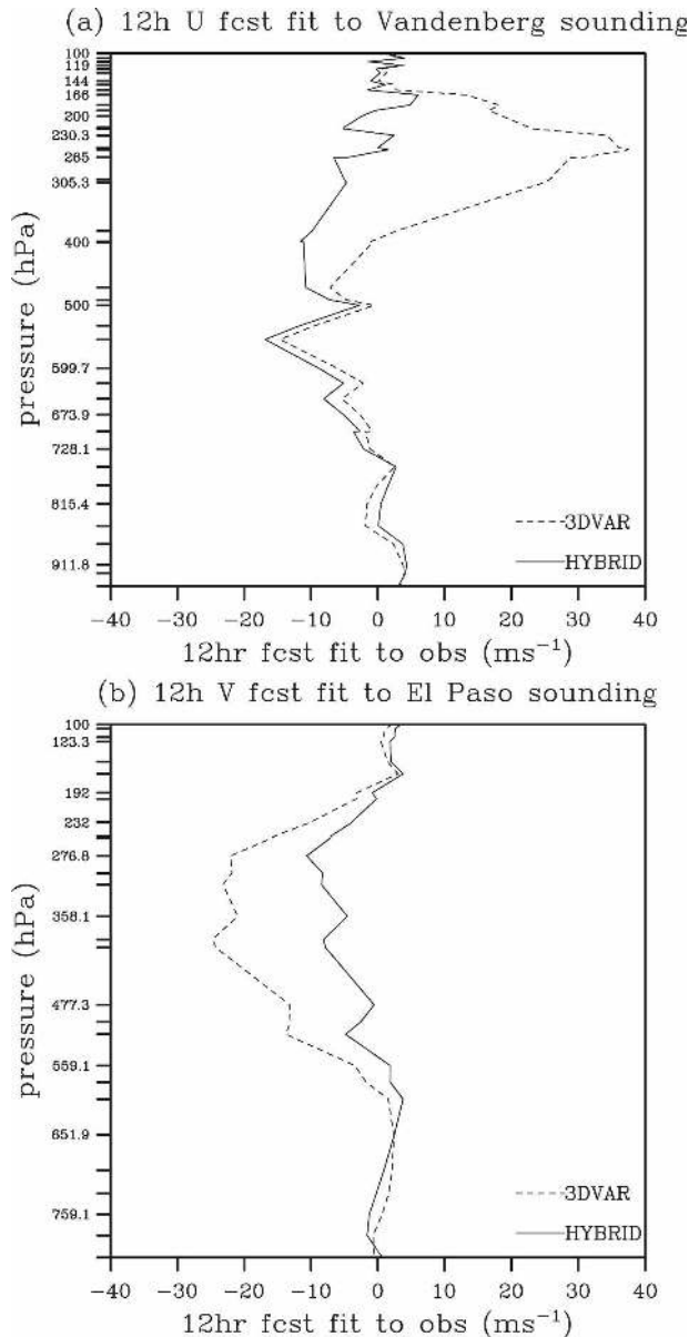
FIG. 8. Fit of the 12-h wind forecast to the soundings valid at 1200 UTC 9 Jan 2003 for the 3DVAR (dotted line) and hybrid with 1/\beta_1 = 0.5 and S_e = 2828 km (solid line). (a) Zonal wind fit to the sounding at Vandenberg, CA. (b) Meridional wind fit to the sounding at El Paso, TX.
