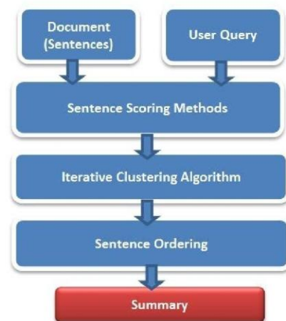
Figure 1. Summarization Process
