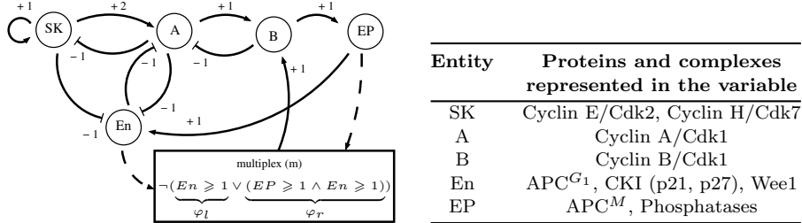
Fig. 4. A simplified 5-variable gene network of the mammalian cell cycle. APC M is a complex involved in surveillance mechanism in order to enter into anaphase (third step of mitosis). The combined effects of the APC G1 , p27 and Wee1 inactivate Cdk1, Cdk2, Cdk4 and Cdk6.
