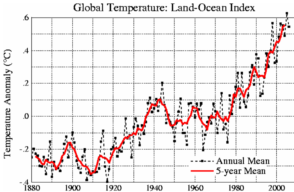
Figure 2.1 Global Annual Mean Surface Air Temperature Change ( www.giss.nasa.gov/data/update/gistemp/graphs )
