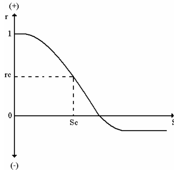
Figure 3.5 Correlation Coefficient ( r ) Versus Distance ( S ) (Liu, 1981).
