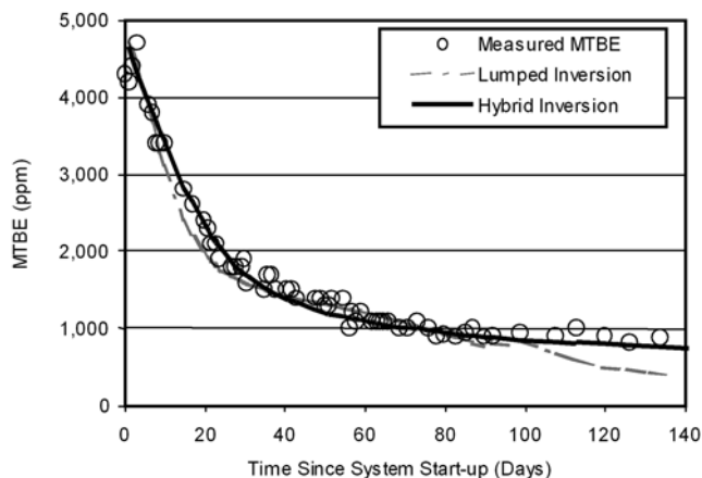
Figure 10. Simulated and observed MTBE concentrations at the IRM well.
