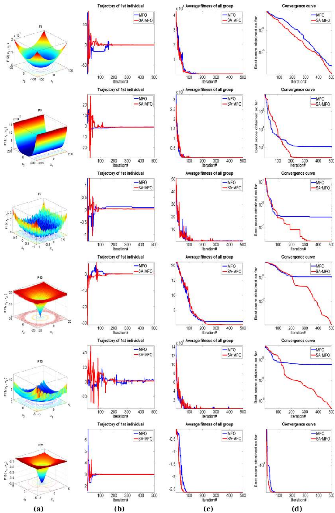
Fig. 3 a Graphical representations of benchmark functions, b the trajectory in first dimension, c the average fitness of all group, and d the convergence curve
