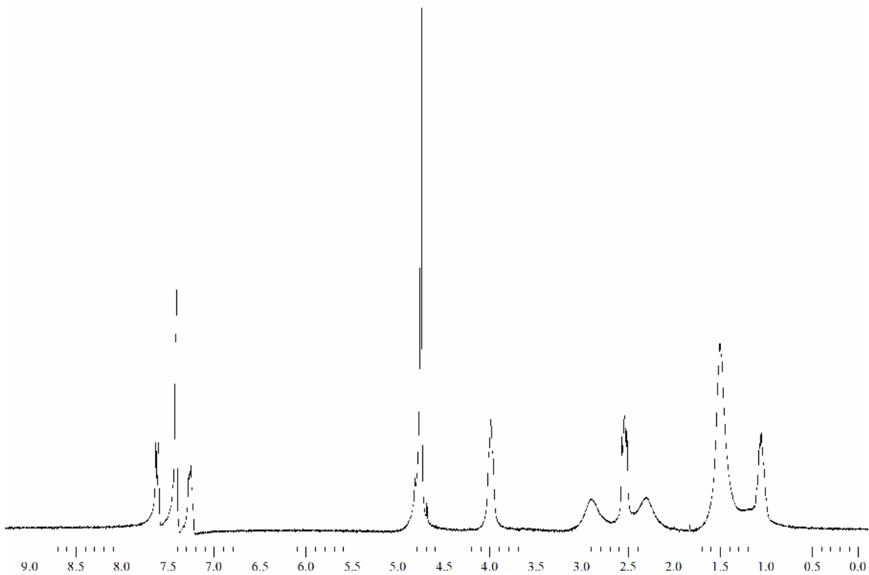
Figure S1: 1 H-NMR spectrum of AZATRUX as a hydrochloride in D 2 O.
