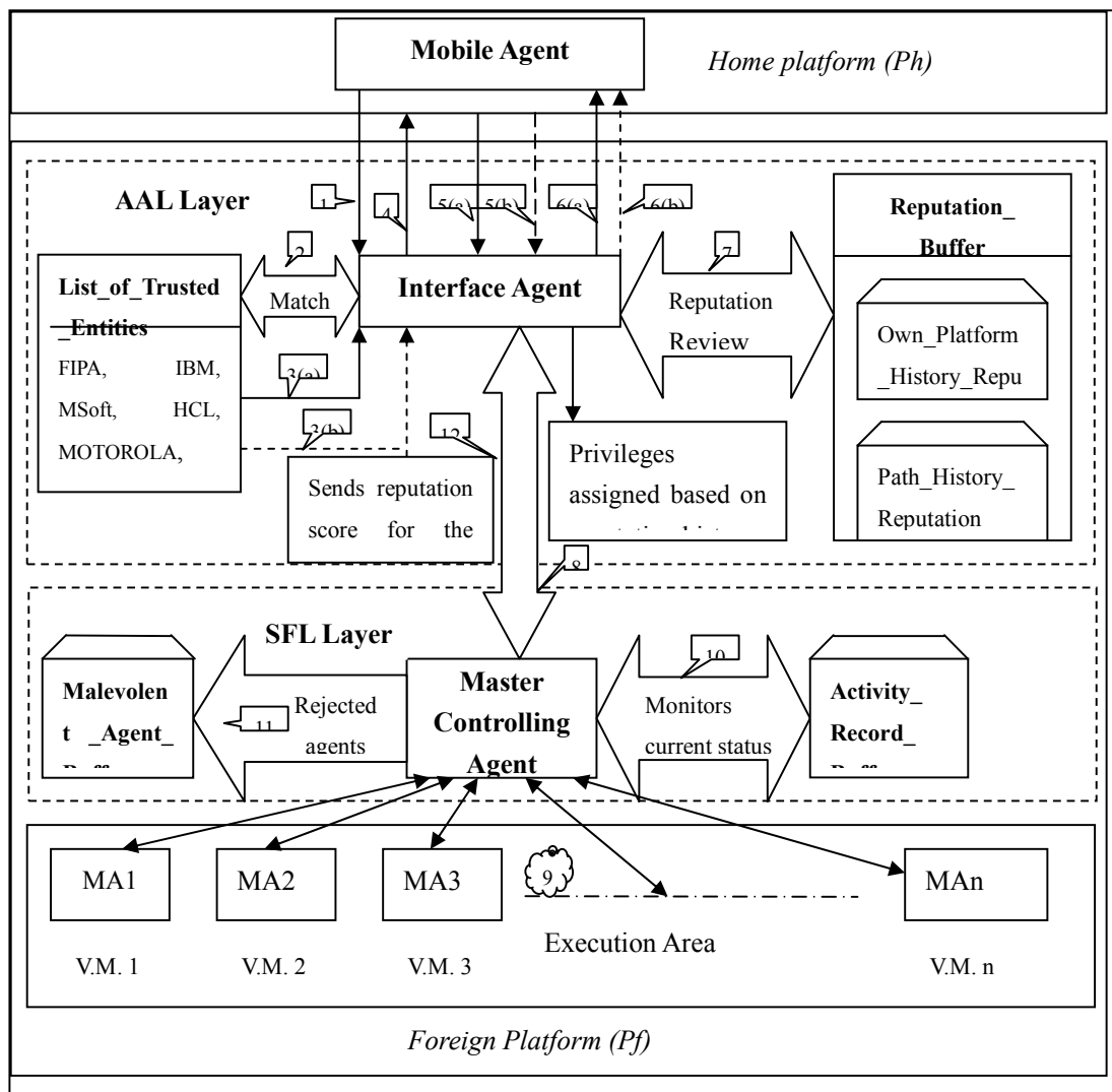
Figure 1: Architecture of the Proposed Platform Security Framework (PSF) [6]
