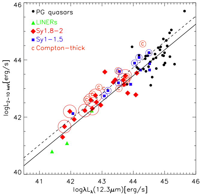
Figure 4. Relationship between 2 and 10 keV unobscured X-ray and 12.3 \mu\text{m} luminosities. The dashed line is the best fit for all Seyfert and LINER galaxies with well-resolved images at 12.3 \mu\text{m} (circled symbols; Gandhi et al. 2009). The solid line is the fit adopted in this paper that is exclusively for PG quasars. It is derived by fixing the slope as that for Seyfert and LINER ones but recalculating the normalization to produce the median trend of PG quasars. The offset between the dashed and solid lines is due to the strong silicate features in the PG quasars. (A color version of this figure is available in the online journal.)
