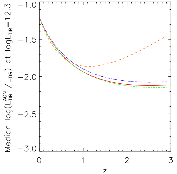
Figure 13. Redshift evolution of the BH energy fraction at L_{\text{TIR}}[L_{\odot}] = 12.3 . Different line styles are for different variants of the model: solid line for reference variant, dashed line for fast_evol_SED_SF, dot-dashed line for low_IR2X_BH, and triple-dot-dashed line for high_IR2X_BH (see Table 1).
