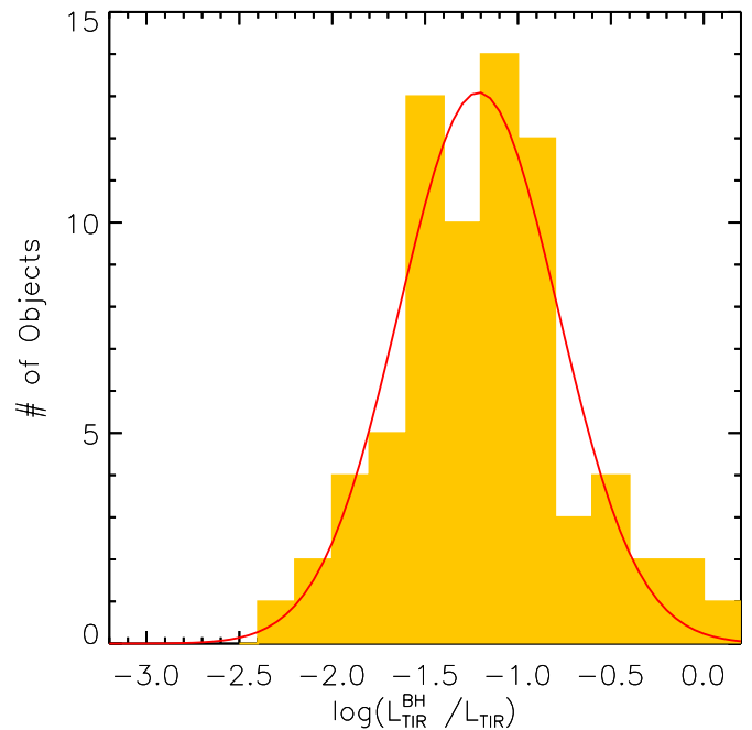
Figure 1. Distribution of the SMBH energy fraction in the total IR band of 74 1 Jy ULIRGs based on the aromatic feature EW measurements by Veilleux et al. (2009). The filled histogram shows the derived SMBH energy fraction distribution. The solid line is the Gaussian fit to the filled histogram. For details, see Section 3.2.
