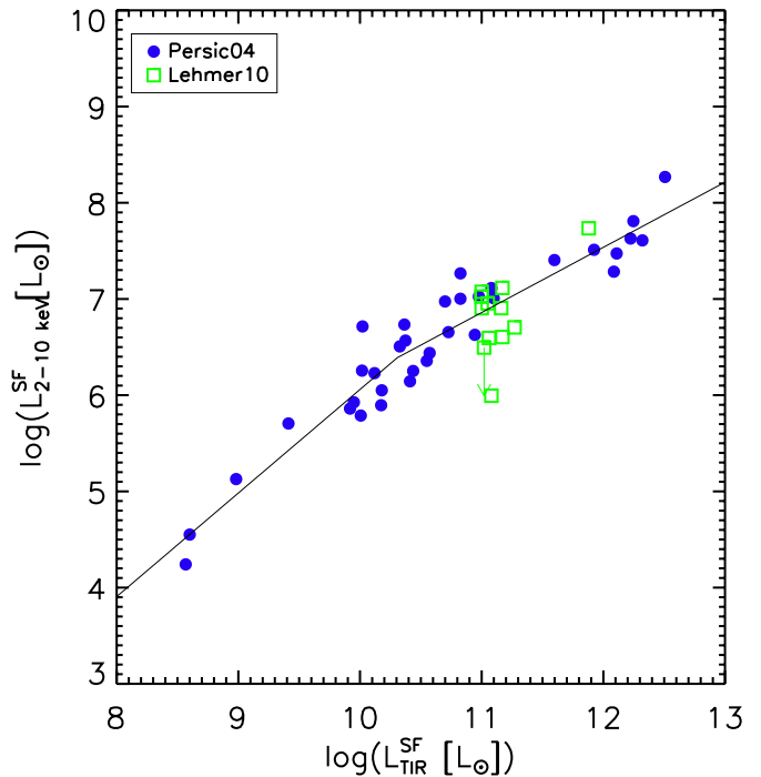
Figure 2. Relationship between IR and X-ray emission of star-forming galaxies based on the sample of Persic et al. (2004) and Lehmer et al. (2010; see Equation (13)).
