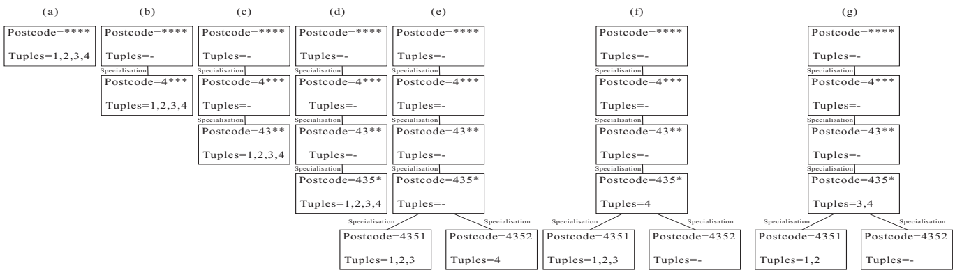
Figure 1: Top-Down Algorithm for Quasi-identifier of Size 1
