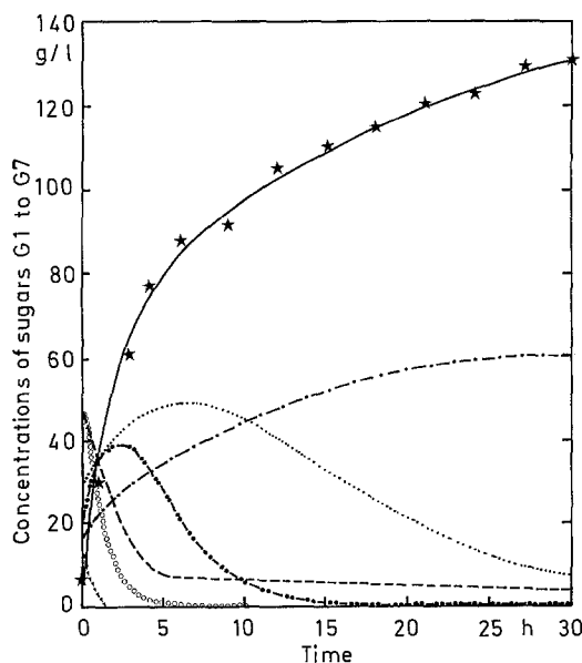
Fig. 3. Calculated profiles (lines) of glucose and other oligosaccharides with DP 2 to DP 7 compared with experimental glucose concentration (★). (—) G_1 ; (---) G_2 ; (···) G_3 ; (-·-·) G_4 ; (- - -) G_5 ; (○○) G_6 ; (▶▶) G_7
