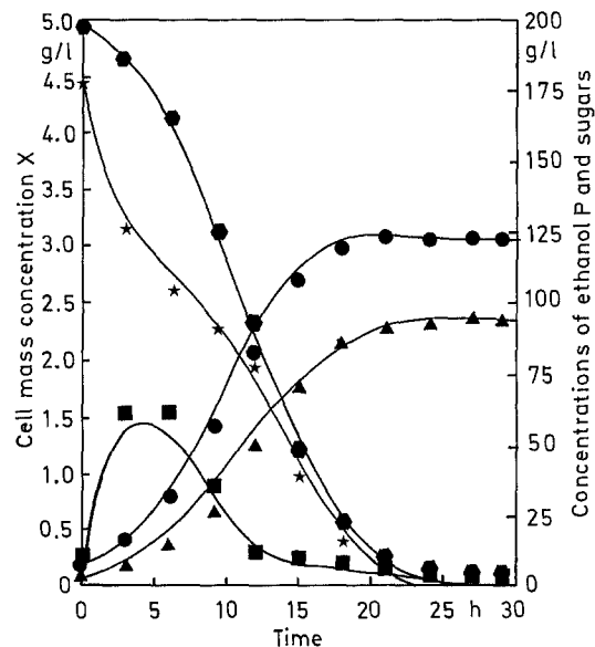
Fig. 8. Comparison of fermentation variables between predicted (lines) and experimental (symbols) SSF process. (▲) ethanol; (●) cell mass; (■) glucose; (●) total sugar; (★)
