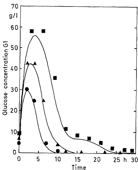
Fig. 7. Effect of initial starch concentration S_0 on simulated (lines) and experimental (symbols) glucose concentration G_1 . S_0 : (●) 100 g/l; (▲) 150 g/l; (■) 200 g/l
