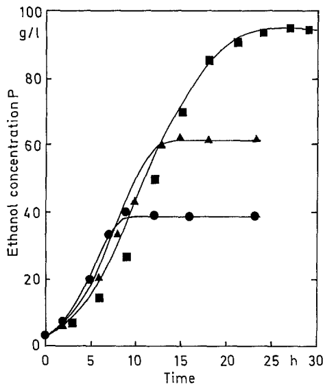
Fig. 6. Effect of initial starch concentration S_0 on simulated (lines) and experimental (symbols) ethanol production P_0 . S_0 : (●) 100 g/l; (▲) 150 g/l; (■) 200 g/l
