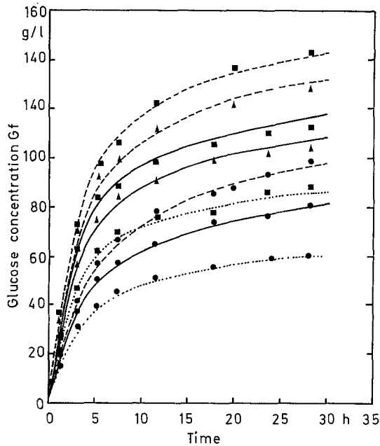
Fig. 4. Profiles of predicted (lines) and experimental (symbols) glucose concentration G_f at various initial starch and AMG concentrations, S_0 and E . Initial starch concentration S_0 : (···) 100 g/l; (—) 150 g/l; (---) 200 g/l. AMG concentration E : (●) 0.2%; (▲) 0.6%; (■) 1.0%
