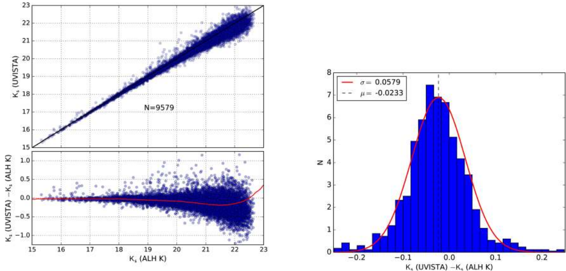
Figure 9. Left-hand panel: UltraVISTA and ALHAMBRA K_s band catalogue photometry comparison for the ALHAMBRA-4 COSMOS field. The right-hand panel shows the distribution of magnitude differences for the bright sample ( 15 < K_s < 19 ), over-plotted with its Gaussian best fit whose parameters are given in the inset.
