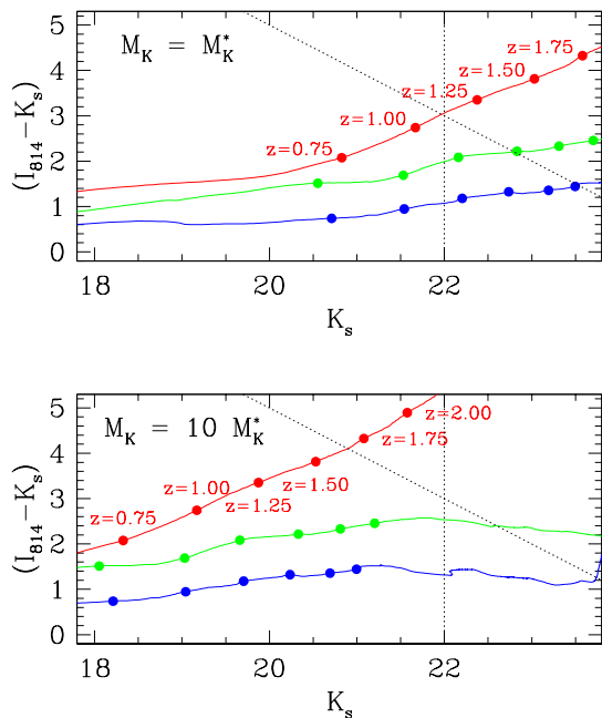
Figure 1. (I_{814} - K_s) versus K_s colour–magnitude diagram. In each plot, the (red, green, blue) (also top, medium, bottom) track corresponds to an (elliptical, spiral, starburst) galaxy template, respectively. Some redshift values are marked on the elliptical template track as a reference.
