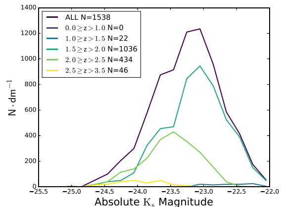
Figure 20. Distribution of the K_s absolute magnitudes in our catalogue for galaxies with (I_{814} - K_s) > 4 and T_B < 5.5 , in different redshift ranges.
