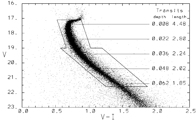
FIG. 1.—Color-magnitude diagram of 46,422 stars from all four WFPC2 CCDs. The box along the main sequence over 17.1 < V < 21.6 shows the selection domain for the 34,091 stars reported herein (PC1 box extended to V = 16.1 ). Numerical entries provide predicted transit depths in magnitudes and duration (central passage) in hours assuming a P_{\text{orb}} = 3.8 day planet with R = 1.3 R_j .
