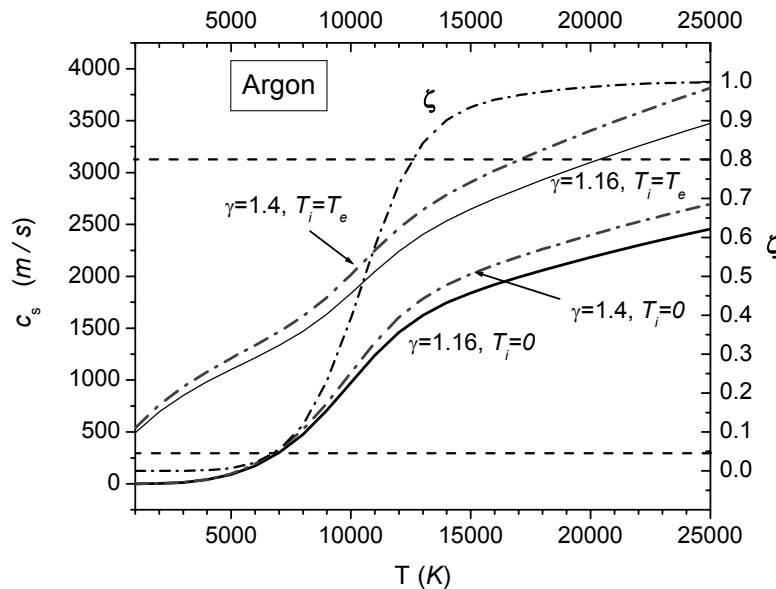
Figure 2.12. Left-axis: Isentropic (non-adiabatic, \gamma=1.16 ) and adiabatic ( \gamma=1.4 ) sound velocity in Ar for hot ( T_i=T_e ) and cold ( T_i=0 ) ion plasmas at different ionization fractions. Right axis, dot-dash curve, ionization fraction. Horizontal lines are placed at the 5% and 80% ionization limits [59]
