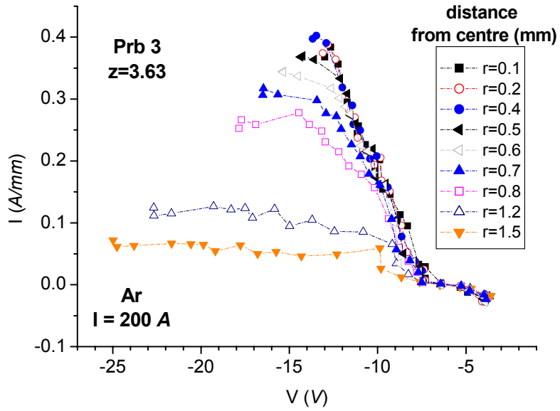
Figure 10.3 a Characteristic curves according to method 4; z=3.63 \text{ mm} , for the 200 A case.
