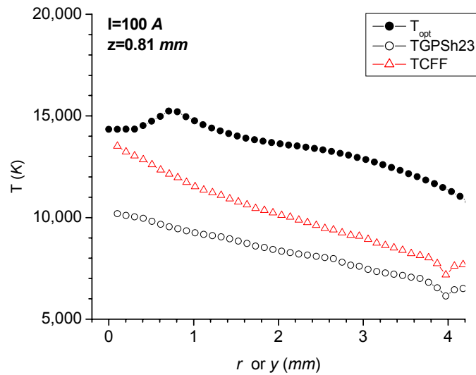
Figure 11.6 c Selection of temperatures for I=100 A. Optical temperatures (full circles) and probe temperatures (empty symbols) at z=0.81 mm
