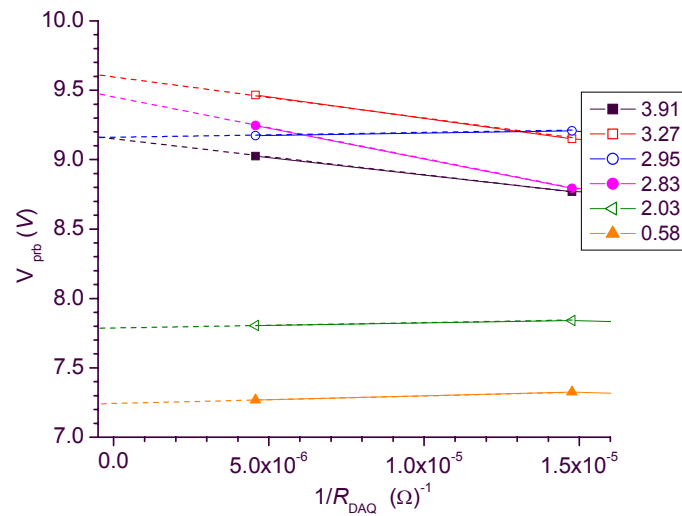
Figure 12.4 b, 50 A, detail of figure 12.3 in the region R_{\text{DAO}} \rightarrow \infty . Six probes of the 11 of figure 12.3
