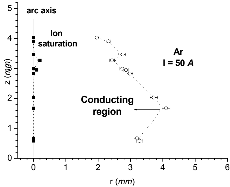
Figure 10.4 a Saturation transition curves for I=50\text{ A} (see text). Full squares: transition between ion non-saturating (left of curve) and saturating (right of curve) characteristic curves. Empty circles: current carrying region shown for comparison ( cf Chapter 13)
