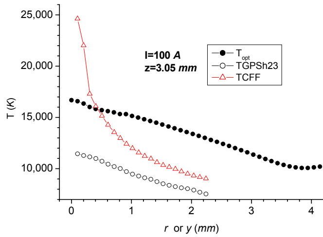
Figure 11.6 d Selection of temperatures for I=100\text{ A} . Optical temperatures (full circles) and probe temperatures (empty symbols) at z=3.05\text{ mm}
