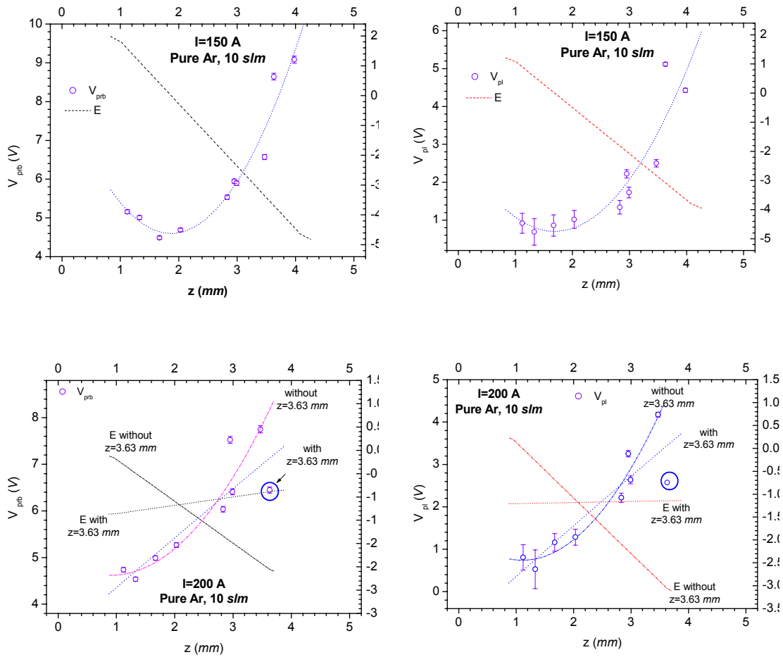
Figure 13.8 Axial probe potential (empty circles with error bar, left axes) and electric field (dot-dashed curve, right axes) for arc currents I=50, 70, 100, 150 and 200\text{ A} . Left column plots represent electric field based on the derivative of the probe measured potential. Plots on the right contain fields determined from the derivative of the plasma potential. The potentials are plotted positively for commodity, whereas the fields are represented with the correct sign. I=200\text{ A} shows different fields (see text).
