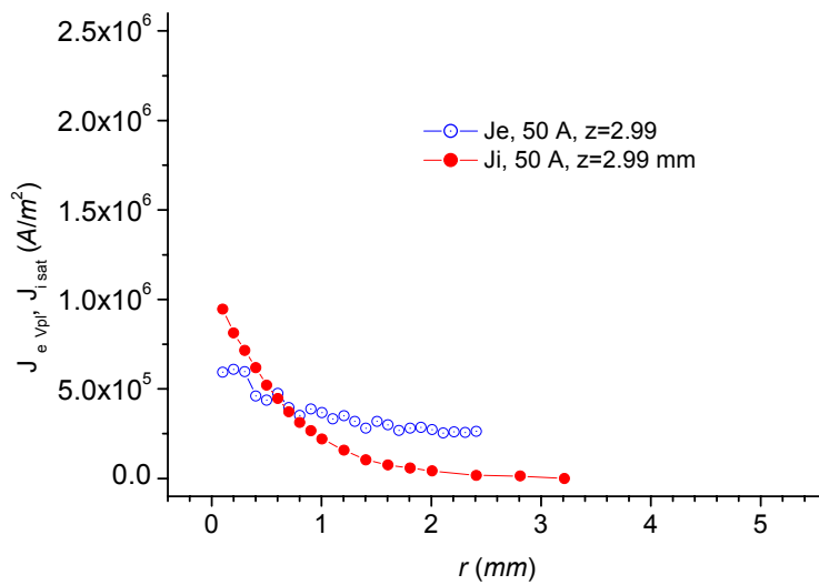
Figure 13.4 b, Arc current 50 A, same as before, z=2.99\text{ mm} from anode
