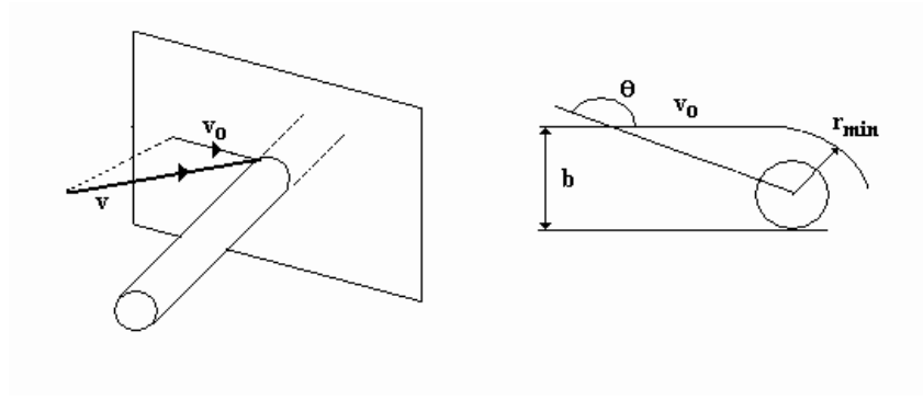
Figure 3.4 Left: projection of the quantities used for spherical probes onto the plane orthogonal to probe axis, used for cylindrical probes. Right: particle deflection by probe potential
