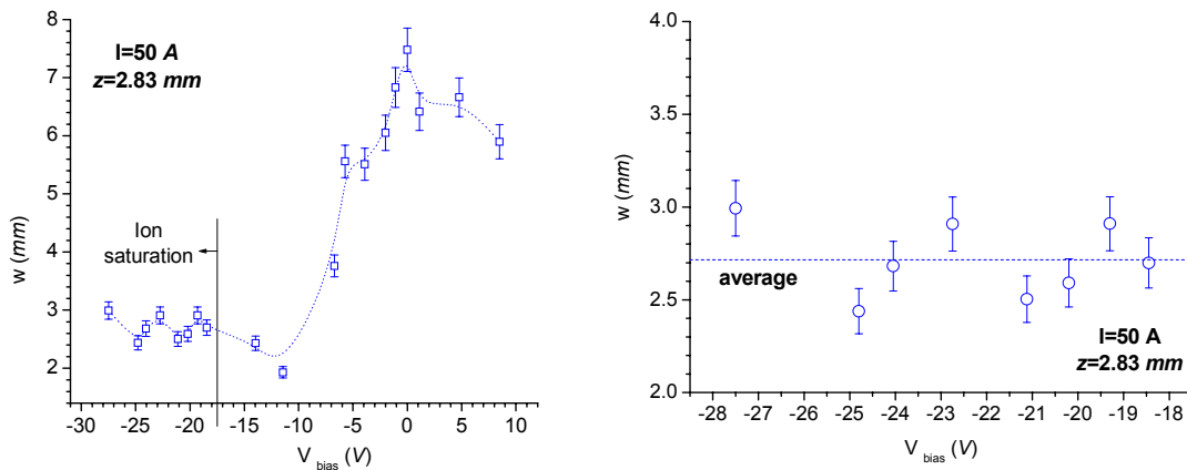
Figure 14.2 I=50\text{ A} , Probe height z=2.83\text{ mm} . Left, comparison between current peak widths for different biases. Right, particular of peak widths at ion saturation
