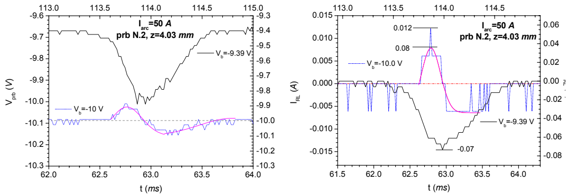
Figure 9.6. I_{\text{arc}}=50 A, probe 2, z=4.03 mm from anode. The two cases close to peak transition (see text). Left, comparison of probe voltages ( V_b=-10 V left axis, V_b=-9.39 V right axis). Right, comparison of currents (same axes)
