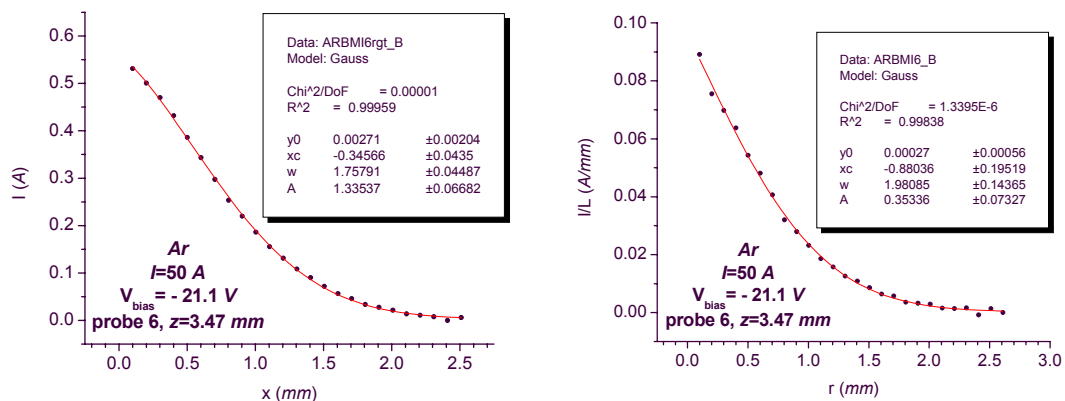
Figure 9.11 Measured (left) and Abel inverted signal (right) obtained using Nestor Olsen for biased conditions (see text)
