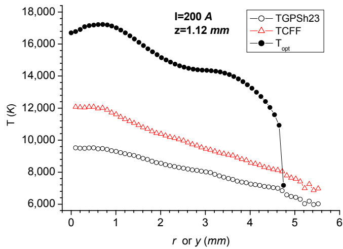
Figure 11.6 e Selection of temperatures for I=200\text{ A} . Optical temperatures (full circles) and probe temperatures (empty symbols) at z=1.12\text{ mm}
