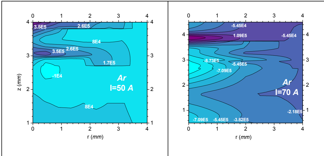
Figure 14.4 Two-dimensional maps for the electron current densities obtained from the currents measured at the plasma potential. I_{\text{arc}}=50 and 70 A
