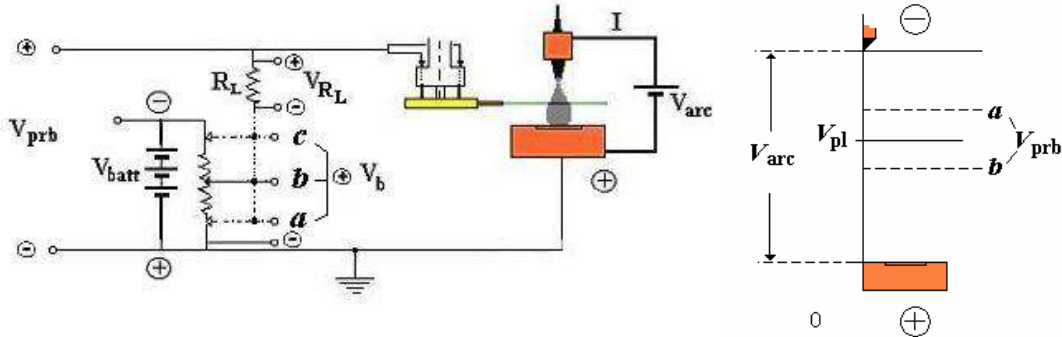
Figure 8.13 Circuit used in biased conditions. Legend: V_{\text{prb}} probe potential; V_{\text{batt}} , constant total battery voltage; R_L , load resistor; V_{RL} fall across load resistor; V_b , applied voltage (bias), measured from a , b or c and earth. Polarity at battery corresponds to 'negative' bias (see text). Polarities indicated by 'small' circles refer to the sign of the voltages as seen at the acquisition channel. Right, some voltage references (see text)
