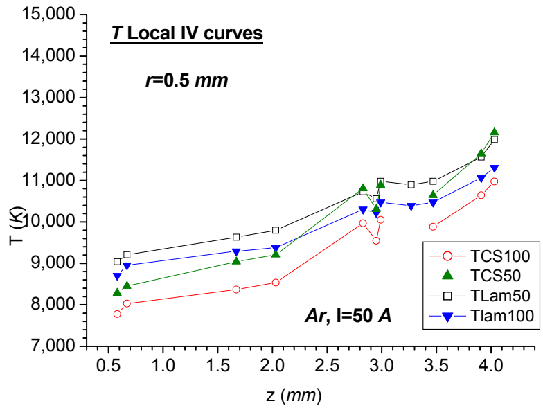
Figure 11.9 c Temperatures obtained from the ion saturation currents parametrized with different but uniform flow velocity and radial distance. r=0.5 \text{ mm} from centre.
