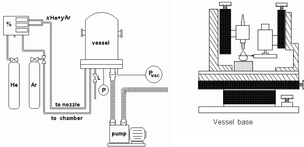
Figure 8.1 Left, the vessel hosting the experimental setup with gas and vacuum feedthroughs, and the gas system. Right, overview of the experimental basement contained in the chamber (“vessel”).
