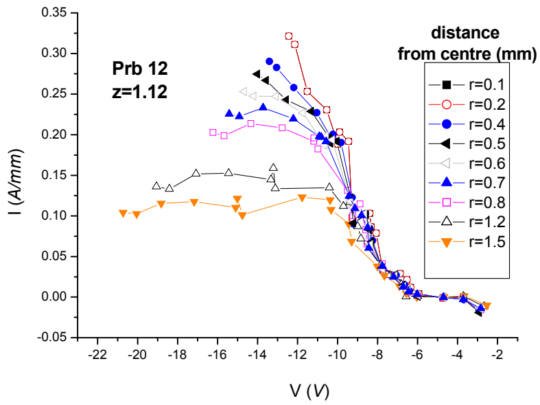
Figure 10.3 c Characteristic curves according to method 4; z = 1.12 \text{ mm} for the 200 A case.
