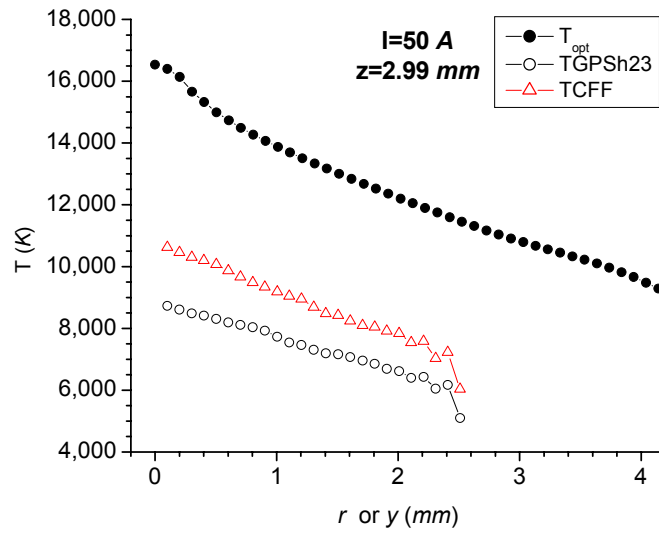
Figure 11.6 b Selection of temperatures for I=50 A. Optical temperatures (full circles) and probe temperatures (empty symbols) at z=2.99 mm
