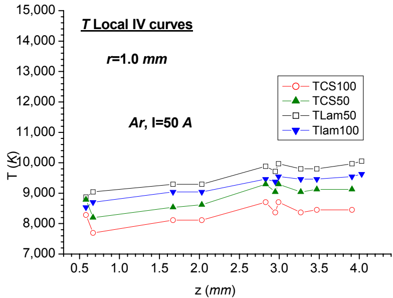
Figure 11.9 d Temperatures obtained from the ion saturation currents parametrized with different but uniform flow velocity and radial distance. r=1.0 \text{ mm} from centre.
