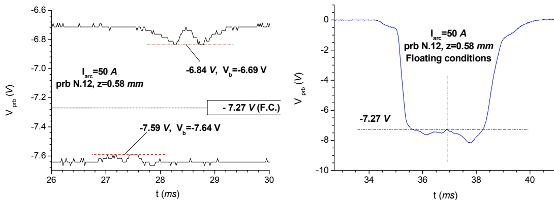
Figure 9.10 I=50 \text{ A} , probe 12, z=0.58 \text{ mm} from anode at V_b=-6.69 \text{ V} and V_b = -7.64 \text{ V} shown together (left). The value obtained from the peak in floating conditions (right) is also indicated
