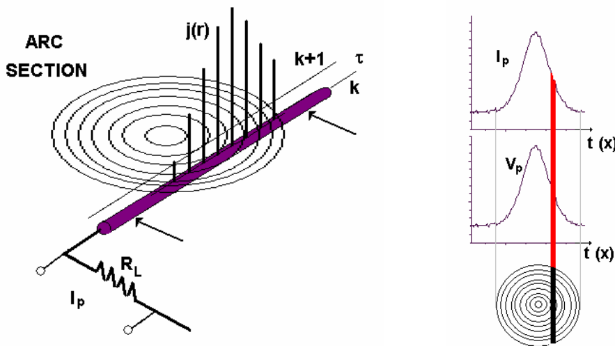
Figure 10.1 for the construction of the V-I curves Left, probe in arc, current distribution on the probe at location k (see text). Right, method 2 ('chordal' averages)
