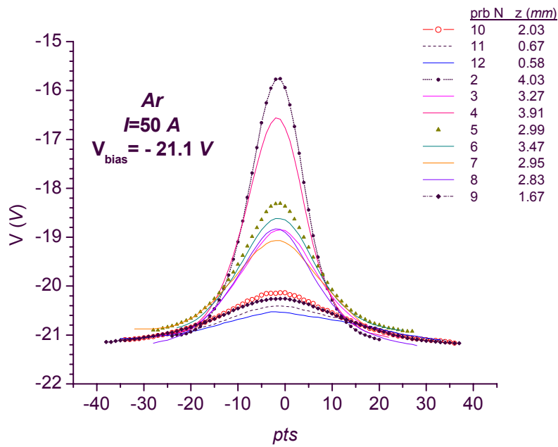
Figure 14.1 a Peak widths. Voltage peaks for all probes under specific bias voltage
