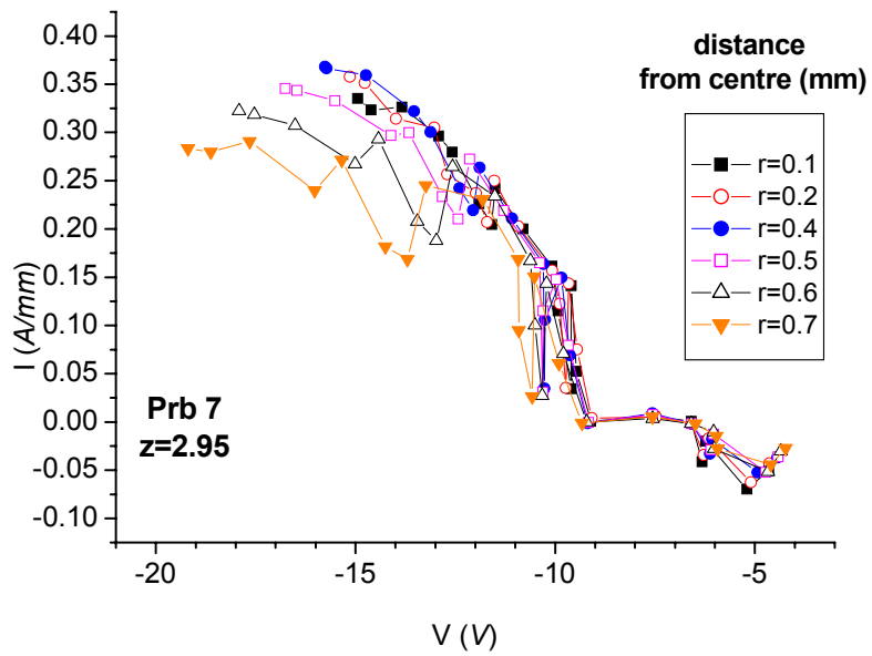
Figure 10.3 b Characteristic curves according to method 4; z= 2.95 \text{ mm} for the 200 A case.
