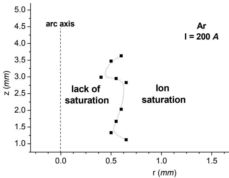
Figure 10.3 d. The transition to ion saturation defined by a radial coordinate exceeding the experimental points, r > r_{\text{sat}} . I = 200 \text{ A}
