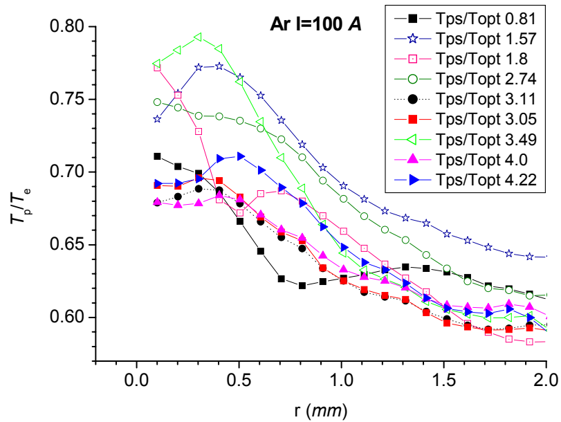
Figure 11.16 b, I=100 A Probe to optical temperature ratios as a function of the radial distance, region 0 to 2 mm
