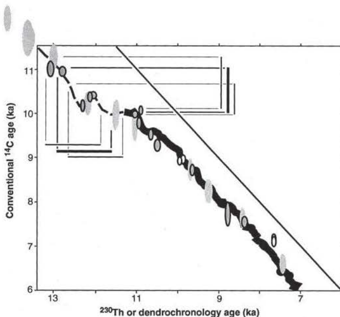
Fig. 4. Plot of ^{14}\text{C} versus ^{230}\text{Th} ages. Ellipses with black outlines are Papua New Guinea data. Of these, stipled ellipses are University of Arizona ^{14}\text{C} analyses and open ellipses are Woods Hole ^{14}\text{C} analyses. Stipled ellipses with no outline are Barbados data (22). The thick black curve represents established and floating dendrochronological ^{14}\text{C} calibrations (2-4). The horizontal bars indicate the timing of the YD, in calendar years, from ice cores (35). The middle horizontal bar is the best estimate of the timing; with errors taken into consideration, the upper horizontal bar is the oldest possible timing and the lower bar is the youngest possible timing. The vertical bars represent corresponding estimates of the timing of the YD in ^{14}\text{C} years, on the basis of the ice-core data and our calibration. The best and the earliest possible estimates agree with other radiocarbon-based estimates of the timing of the YD (35), suggesting that the calibration is accurate. The latest possible estimate for the start of the YD is later than other radiocarbon-based estimates, which suggests that the latest possible ice-core estimate is too young. The Papua New Guinea data define a 1280-year interval between 12.3 and 11.0 ka over which ^{14}\text{C} ages changed by only 210 years. This period was coincident with the period of reduced melting (Figs. 2 and 3). A decrease in atmospheric ^{14}\text{C}/^{12}\text{C} (Fig. 5) caused the compression of the ^{14}\text{C} time scale during this period.
