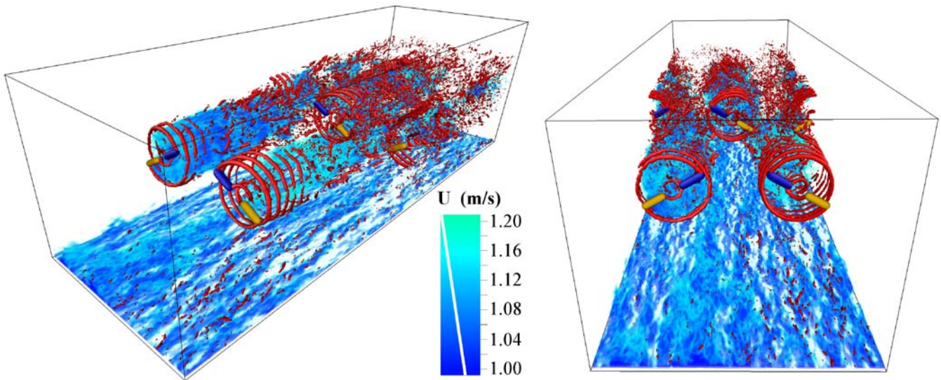
Fig. 7 Instantaneous views of the flow field from Case J with staggered counter-rotating turbines. Resolved streamwise velocity is volume rendered, and the colors correspond to different flow speeds, as shown in the color scale. The white line on the color scale indicates opacity of the volume rendering. The blue end of the scale is more opaque than the aqua end. The red isosurfaces are a positive value of the second invariant of the velocity-gradient tensor, denoting the locations of vortices. The purple and yellow isosurfaces are positive and negative values of the vertical component of the body force, respectively, created by the actuator lines. The view at left is from upwind and offset laterally. The view at right is from upwind. Cross-stream domain boundaries are periodic.
