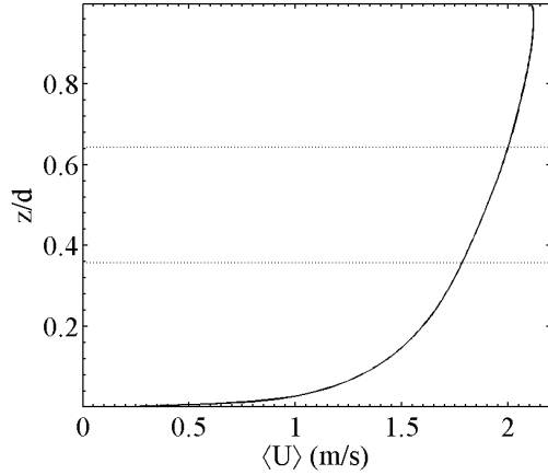
Fig. 2 Mean horizontal velocity profile of tidal channel precursor flow.
