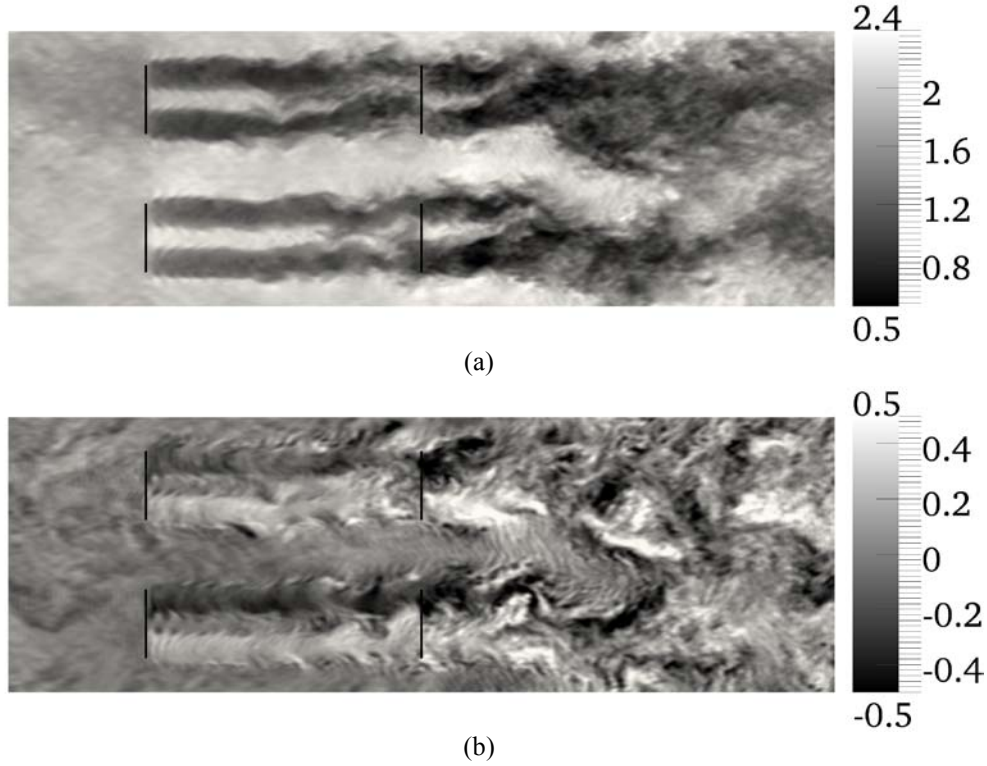
Fig. 8 Instantaneous contours of (a) resolved streamwise velocity and (b) resolve vertical velocity in a horizontal plane at the turbine hub height from Case B. The flow is from left to right, the black vertical lines denote the location of the rotor disks, and the units are m/s.
