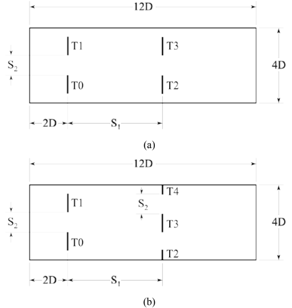
Fig. 1 Plan view of tidal turbine array in (a) non-staggered and (b) staggered configuration. Flow is from left to right.
