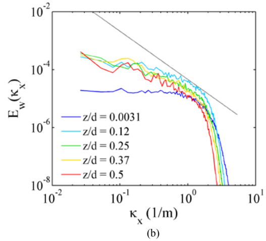
Fig. 5 One-dimensional spectra taken in the streamwise direction of (a) horizontal velocity and (b) vertical velocity at various heights.
