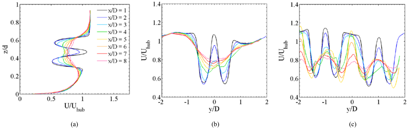
Fig. 9 Time-averaged resolved streamwise velocity profiles in the wakes of the tidal turbines. Vertical profiles aligned with the turbine centerline from Case A are shown in (a). Horizontal profiles at hub height from Case A and Case I are shown in (b) and (c), respectively.
