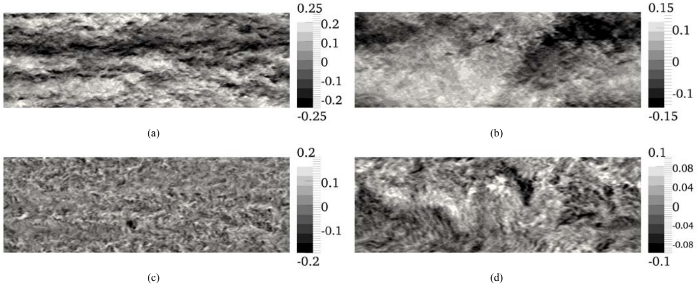
Fig. 6 Contours of instantaneous resolved velocity normalized by hub height velocity on horizontal planes. Contours (a) and (b) are of streamwise velocity, \bar{u} / U_{hub} , and (c) and (d) are of vertical velocity, \bar{w} / U_{hub} . Contours (a) and (c) are at z/d = 0.1 , and contours (b) and (d) are at z/d = 0.5 . Flow is from left to right.
