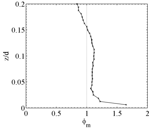
Fig. 3 Non-dimensional velocity shear profile of tidal channel precursor flow.
