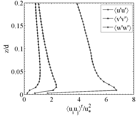
Fig. 4 Normalized velocity variances of the tidal channel precursor flow.
