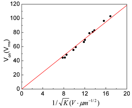
FIG. 4. (Color online) Linear fit of V_{\text{on}} vs 1/\sqrt{K} according to Eq. (6) with A=5.92 \mu\text{m}^{1/2} , \lambda=633 nm.
