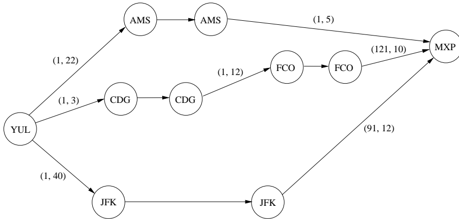
Figure 2: An example graph G_{si}
