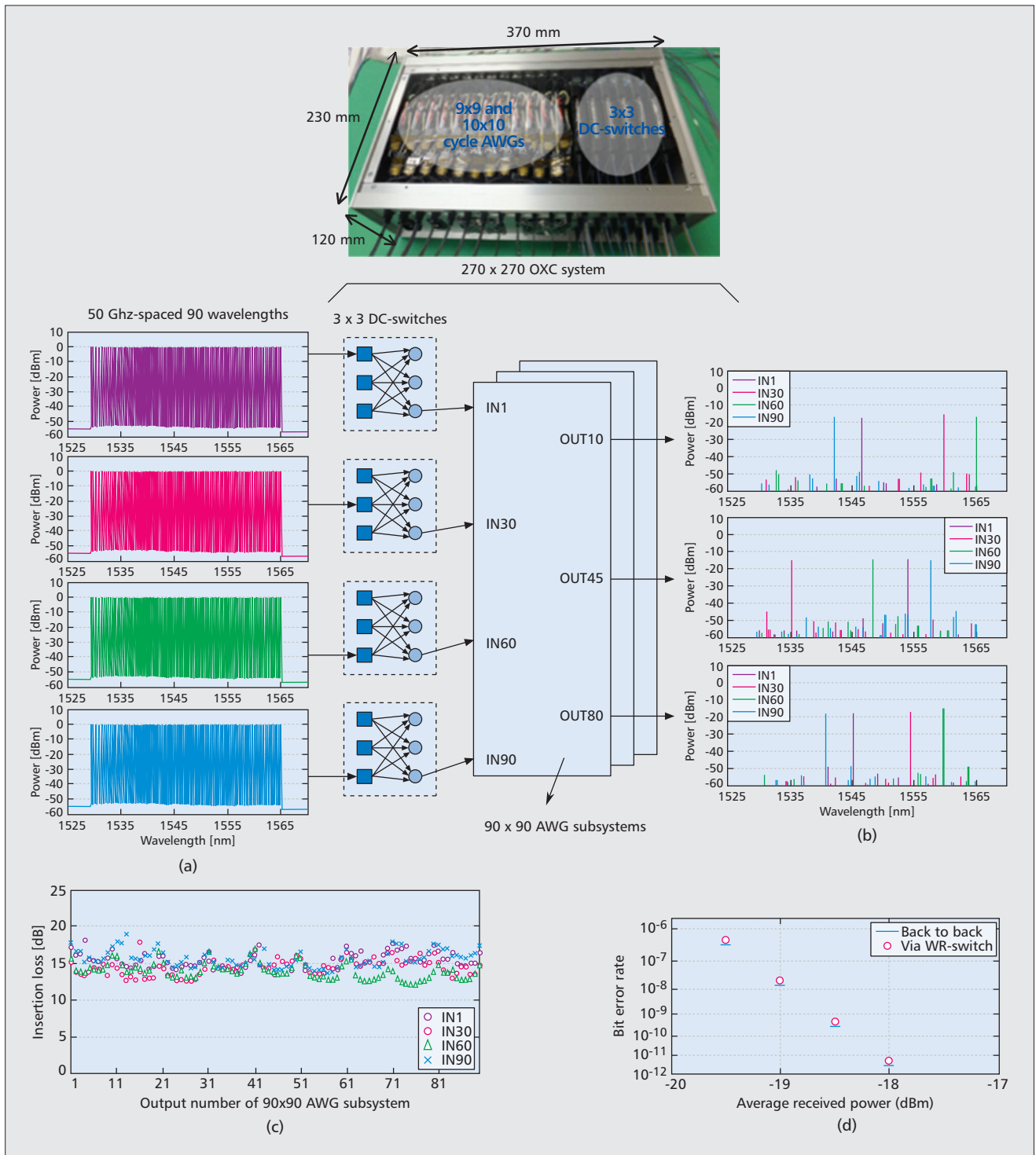
Figure 5. Experiment on developed 270 × 270 OXC system: a) input signals; b) output signals; c) insertion loss; d) measured bit error rate (1550.111 nm).
