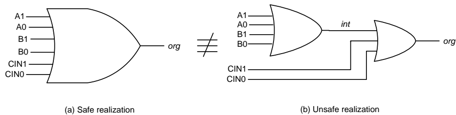
Fig. 6 Naïve decomposition of the 6-input OR gate, potentially causing a gate orphan
