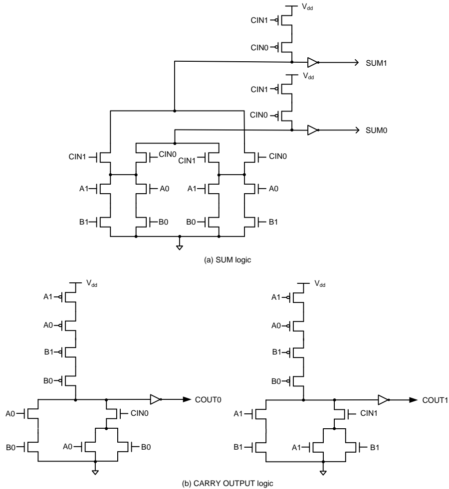
Fig. 4 Martin's weak-indication full adder
