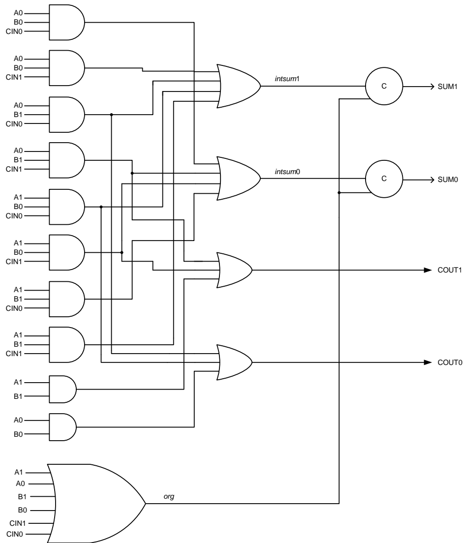
Fig. 5 Seitz's weak-indication full adder
