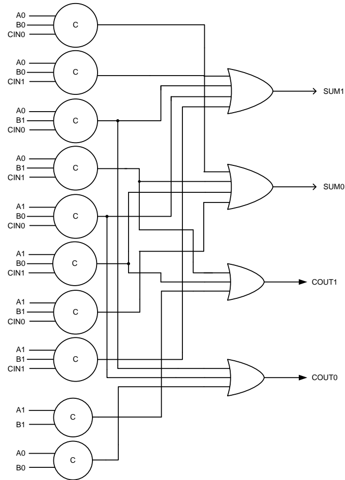
Fig. 3 DIMS weak-indication full adder
