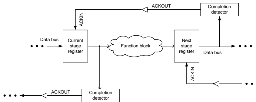
Fig. 1 Standard self-timed system architecture employing delay-insensitive data encoding and 4-phase handshaking
