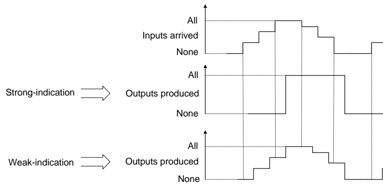
Fig. 2 Input-output behavior of strong and weak-indication function blocks
