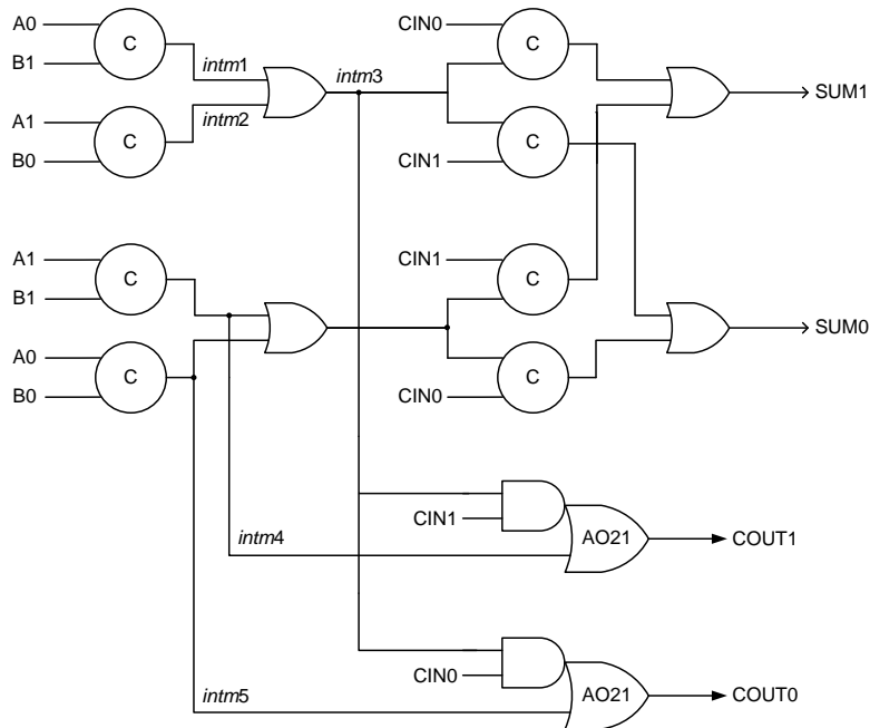
Fig. 7 Proposed weak-indication full adder
