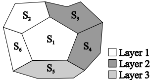
Fig. 3. Hypothesis testing. The segment S_1 has 5 neighbouring segments assigned to the layers 1, 2 and 3 which we call the neighbouring layers of S_1 . We avoid testing layer 1 on S_1 , since this is the current assignment. The layer hypotheses of layer 2 and 3 need to be checked. We point out that although there may be a large number of neighbouring segments, the layer neighbourhood is usually very small, which is a major argument for the algorithm’s efficiency.
