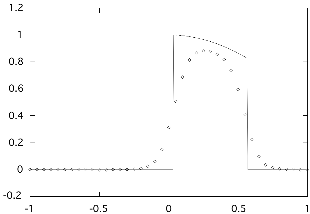
Figure 13: Plot of WENO5 shock capturing solution at x = 0.5, t = 1 with N_x = N_y = 40 , ◇, and exact solution, solid line.
