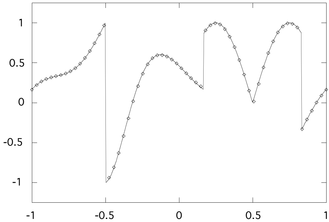
Figure 3: Plot of WENO5 level set tracking solution at t = 2 with N_x = 61 , \diamond , and exact solution, solid line.
