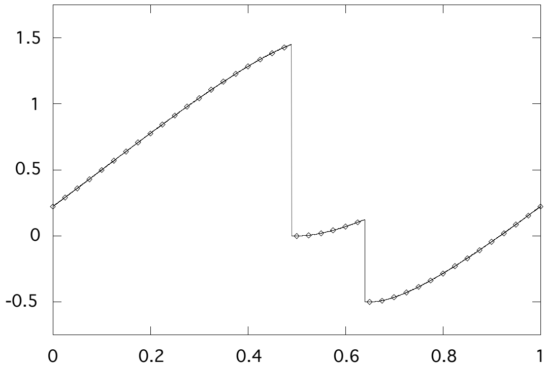
Figure 6: Plot of WENO5 level set tracking solution at t = 0.2 with N_x = 40 , \diamond , and converged level set tracking solution ( N_x = 2560 ), solid line.
