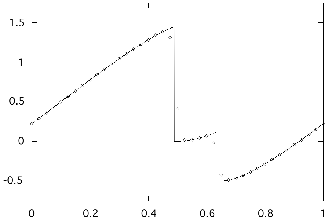
Figure 5: Plot of WENO5 shock capturing solution at t = 0.2 with N_x = 40 , \diamond , and converged level set tracking solution ( N_x = 2560 ), solid line.
