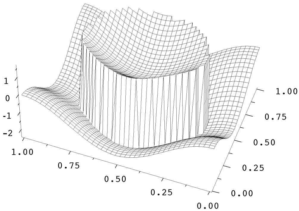
Figure 8: Surface plot of WENO5 level set tracking solution at t = 1 with N_x = N_y = 40 .
