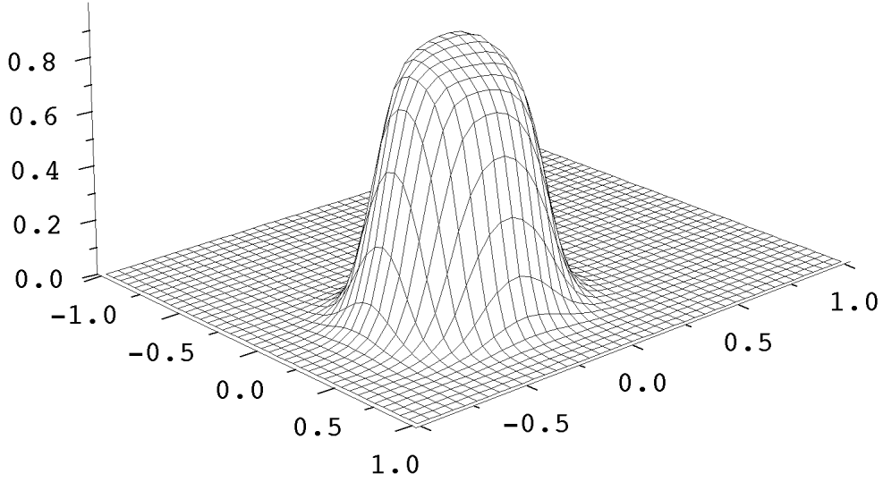
Figure 11: Surface plot of WENO5 shock capturing solution at t = 1 with N_x = N_y = 40 .
