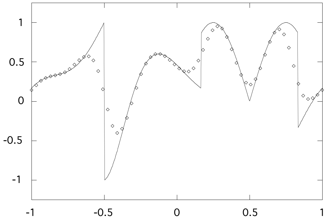
Figure 2: Plot of WENO5 shock capturing solution at t = 2 with N_x = 61 , \diamond , and exact solution, solid line.
