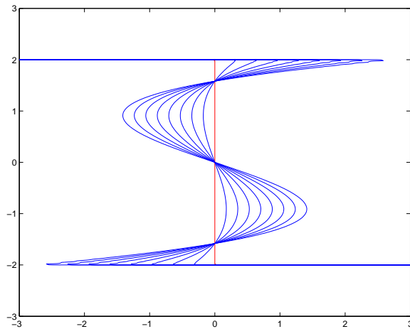
FIGURE 2. Our approach applied to a Riemann problem, with initial step function, that produces multi-valued solutions. The plots are at 0.1160138 time intervals with the final curve at time 0.928111
