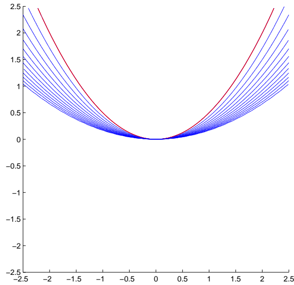
FIGURE 3. Our approach for free motion on an initial parabola, the one above the rest. No singularities appear in this example. The plots are at time intervals of 0.167318 with the final curve at time 2.00781.
