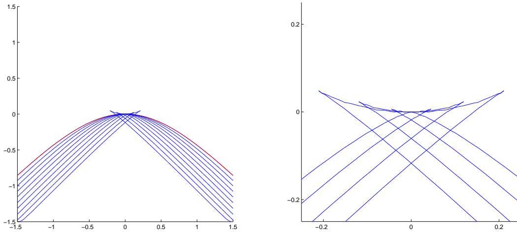
FIGURE 5. Our approach capturing caustics, with a swallow-tail multi-valuedness developing at the critical time with initial curve the uppermost concave down parabola. The plots are at time intervals of 0.1673176 with the final curve at time 1.50586. The figure on the right is a zoomed picture around the singularity of the solutions at and after the critical time.
