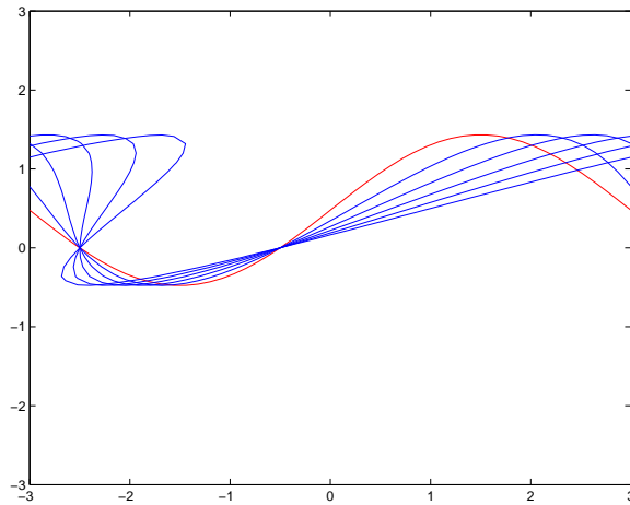
FIGURE 1. Our approach capturing an initial sine function overturning to become multi-valued. The plots are at 0.3921268 time intervals, with the final curve at time 1.96063.
