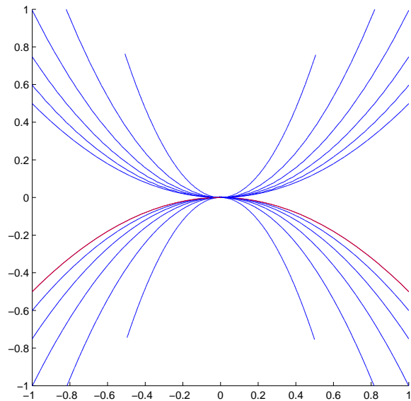
FIGURE 4. Our approach showing focusing on an initial inverted parabola, the uppermost concave down one. The parabola remains concave down and adds curvature before the singularity, after which it switches to concave up and relaxing in curvature. The plots are at time intervals of 0.1669248 with the final curve at time 2.0031.
