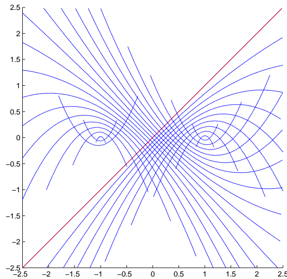
FIGURE 6. Our approach for the harmonic oscillator showing oscillating focusing effects occurring between two points. The initial curve is the line through the origin of slope 1. This subsequently bends into concave down parabolas, then concave up ones about the singularity on the right. In later time these straighten out to a line of slope -1 and reproduce the behavior about the singularity on the left. The plots are at time intervals of 0.333484 with the final curve at time 10.0045.
