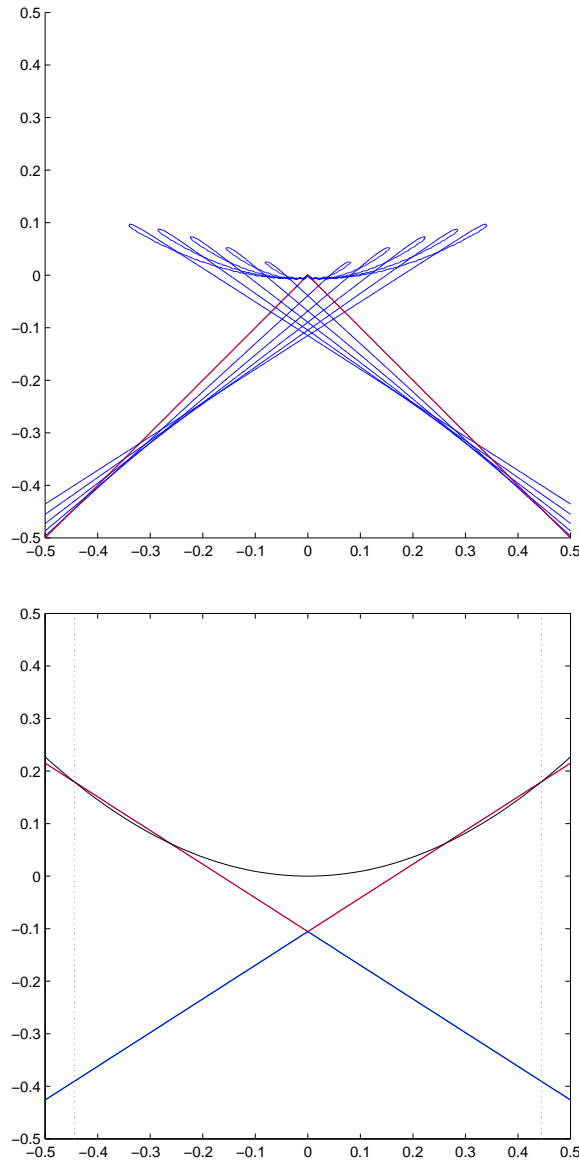
FIGURE 7. Our approach applied in the semi-classical limit for plasma is shown. The initial curve, the inverted V-shape, develops a swallow-tail with small, thin loops at the ends. The plots are at time intervals of .0888888 with the final curve at time 0.444444. The figure on the right shows branches of the exact solution with the same characteristics as in the computed solution.
