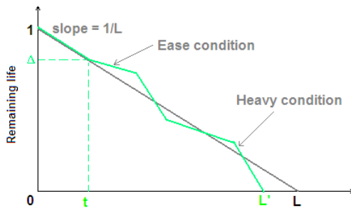
Figure 12. Graph of remaining life against time
