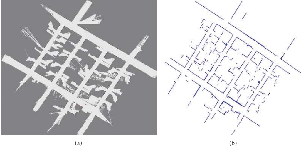
FIGURE 14: Mapping results of intel_oregon using (a) general RBPF SLAM (grid map) and (b) proposed lightweight SLAM (line segment map).
