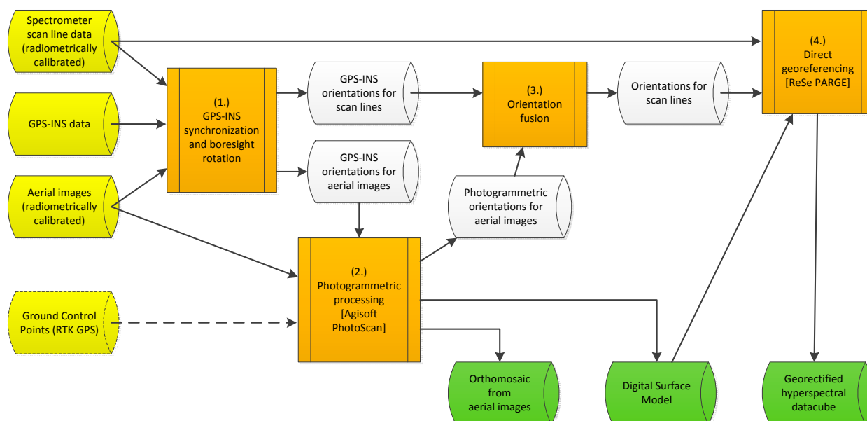
Figure 3. Flowchart of the HYMSY geometric processing chain. The radiometric (reflectance factor) processing (Section 3.1) is done prior to geometric processing. The yellow cylinders are input data, white cylinders are temporary data, and green cylinders are final output data products. Orange boxes are processing steps.
