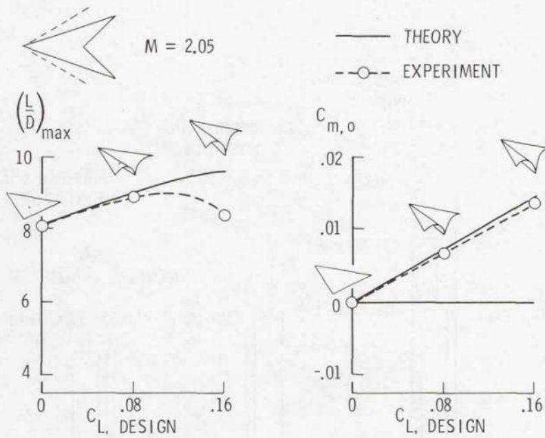
Figure 4.- Example of wing design for drag minimization.
