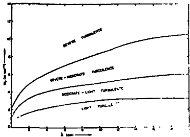
Fig. 22. Forecast degree of CAT. When the maximum vertical velocity in the lee wave is determined from Eq. 25 and the lee wavelength is determined from \lambda = 2\pi/k , the degree of CAT can be determined from this graph (after Foltz, 1967).
