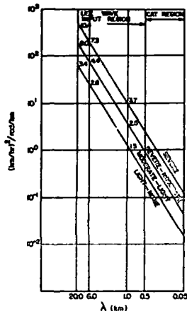
Fig. 23. Spectra of lee wave energy. The values entered on the spectral curves of -5/3 slope are the maximum vertical velocities contained in the lee waves in m \text{ sec}^{-1} at the lee wavelength necessary to result in the level of energy ( w component) in the CAT wavelength region to cause various degrees of CAT (after Foltz, 1967).
