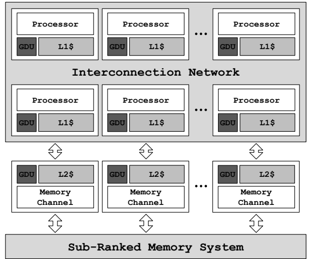
Figure 4: The proposed LAMAR GPU architecture. Each on-chip cache is sectored and is augmented with a GDU; off-chip memory is sub-ranked in order to allow fine-grained accesses.
