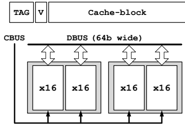
Figure 2: The baseline memory hierarchy using a CG -only memory system with a 64-byte ( 64b \times 8 -bursts) minimum access granularity per channel. CBUS and DBUS represent the command and data bus, respectively.
